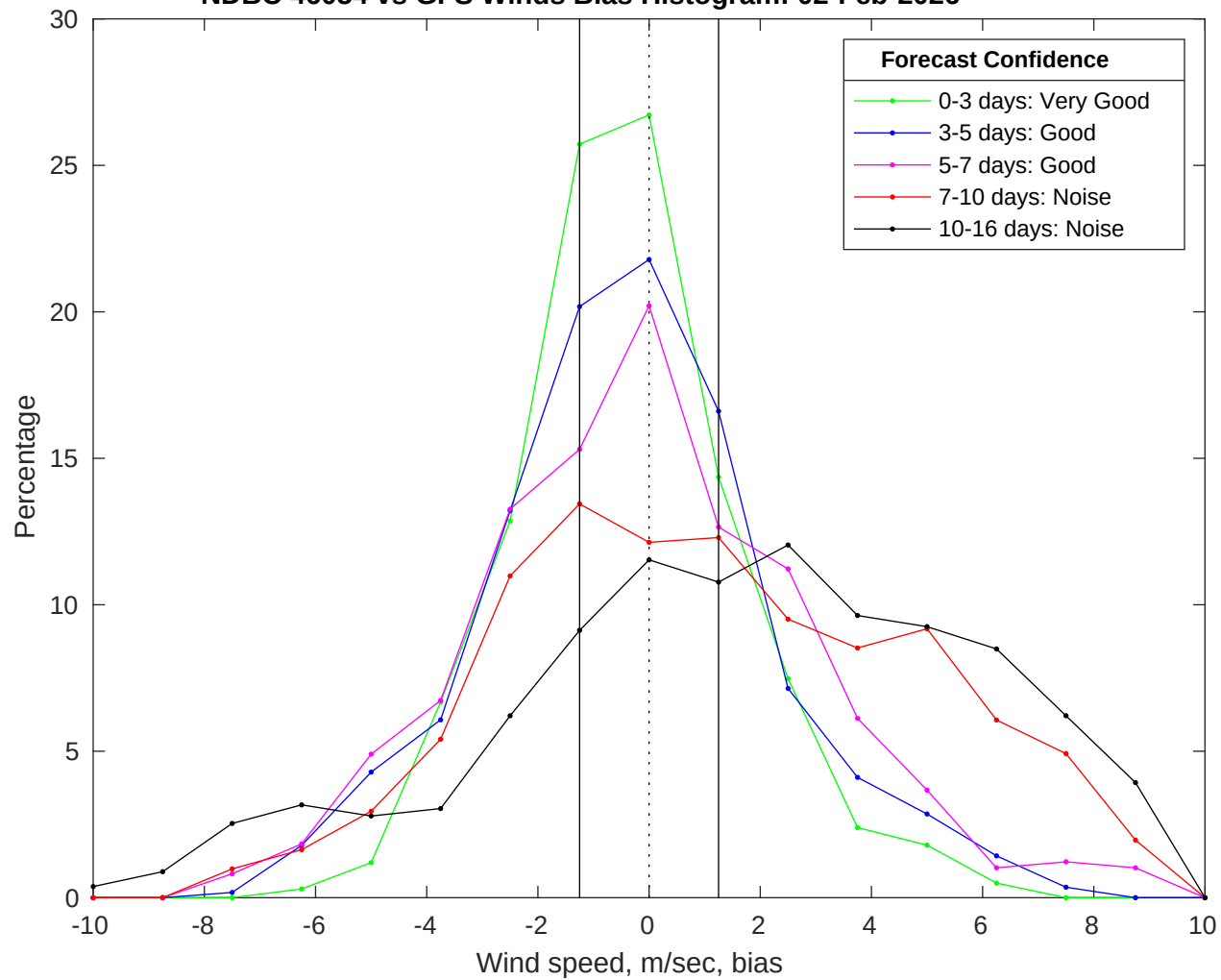
NDBC 46054 vs GFS Winds Bias Histogram: 02-Feb-2026
