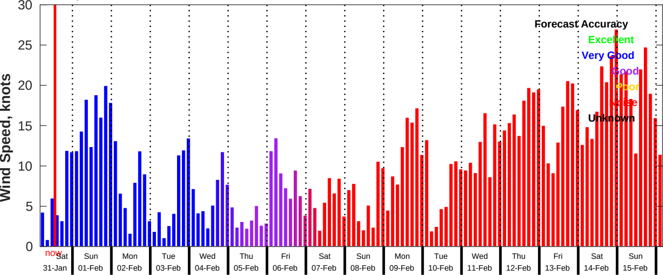
GFS Wind Speed Forecast for NDBC 46054 from 31-Jan-2026 04:00:00 to 16-Feb-2026 04:00:00
