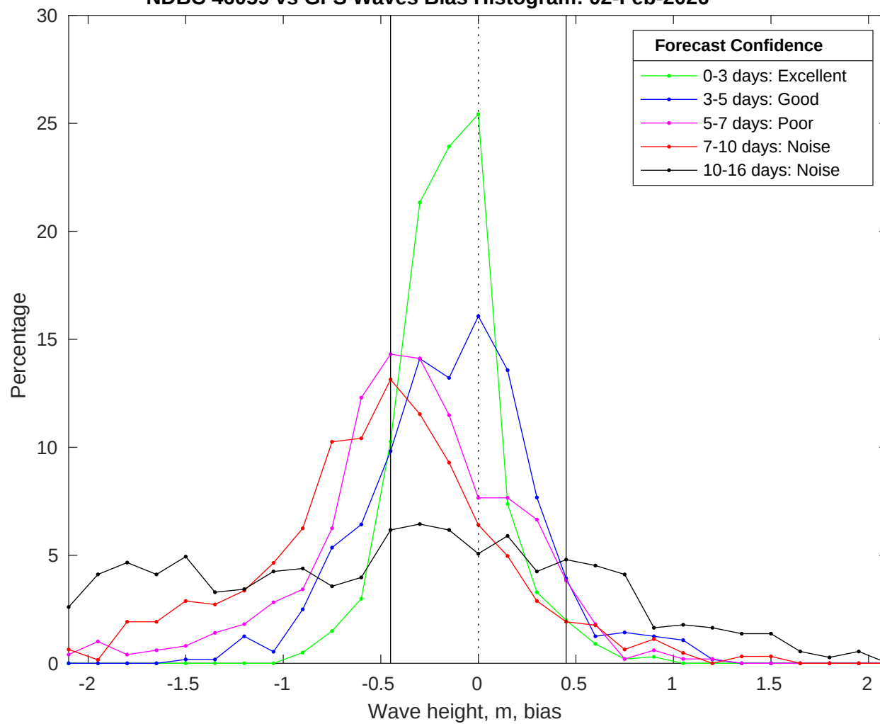
NDBC 46059 vs GFS Waves Bias Histogram: 02-Feb-2026
