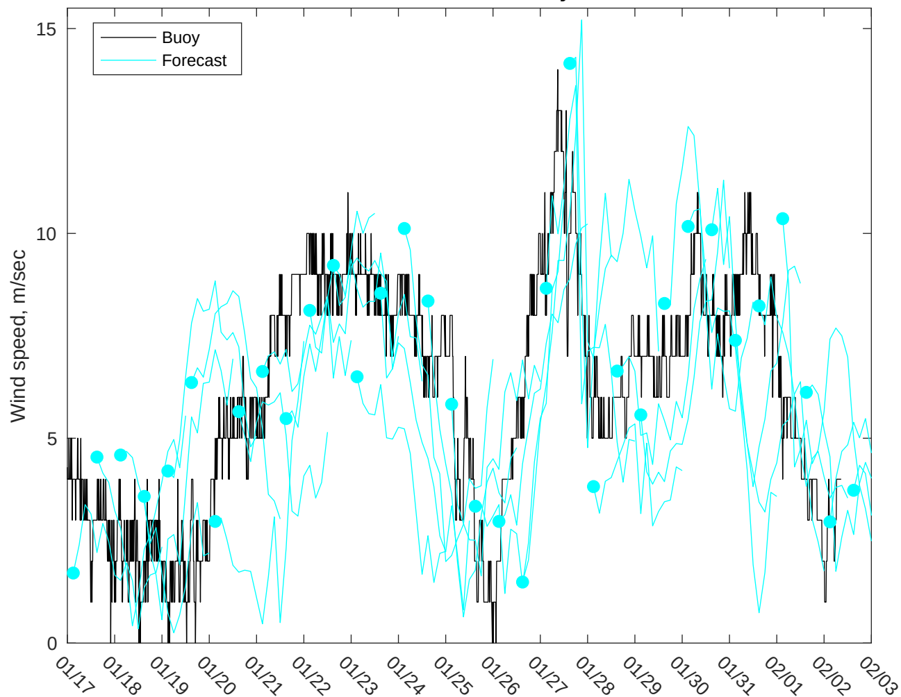
NDBC 46059 vs GFS Winds: 5 to 7 day forecast
