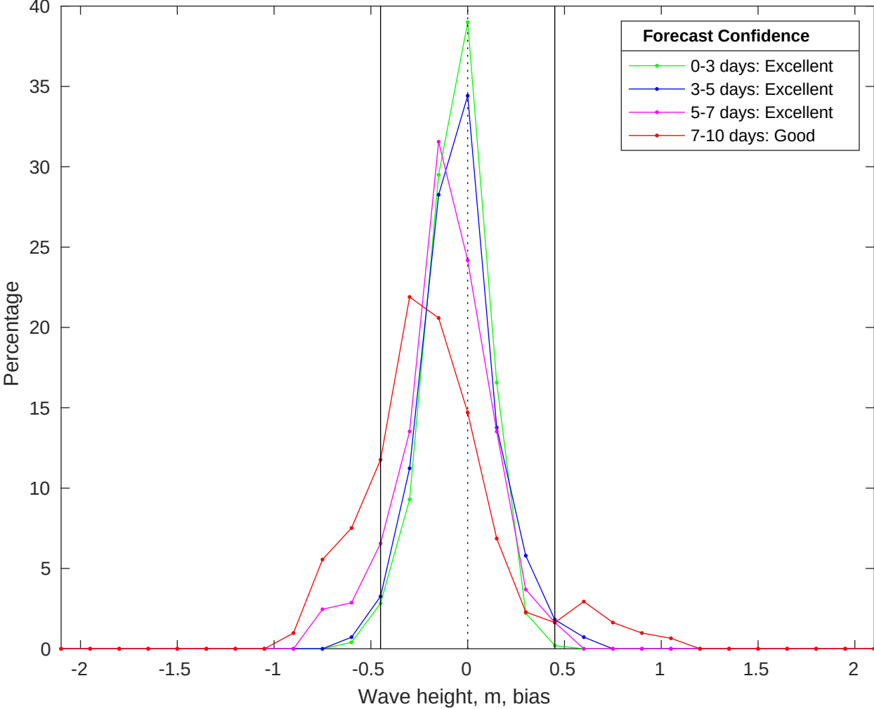
NDBC 46069 vs CMEMS Waves Bias Histogram: 31-Jan-2026
