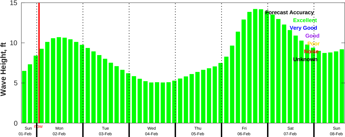
CMEMS Wave Forecast for NDBC 46069 from 01-Feb-2026 16:00:00 to 08-Feb-2026 16:00:00
