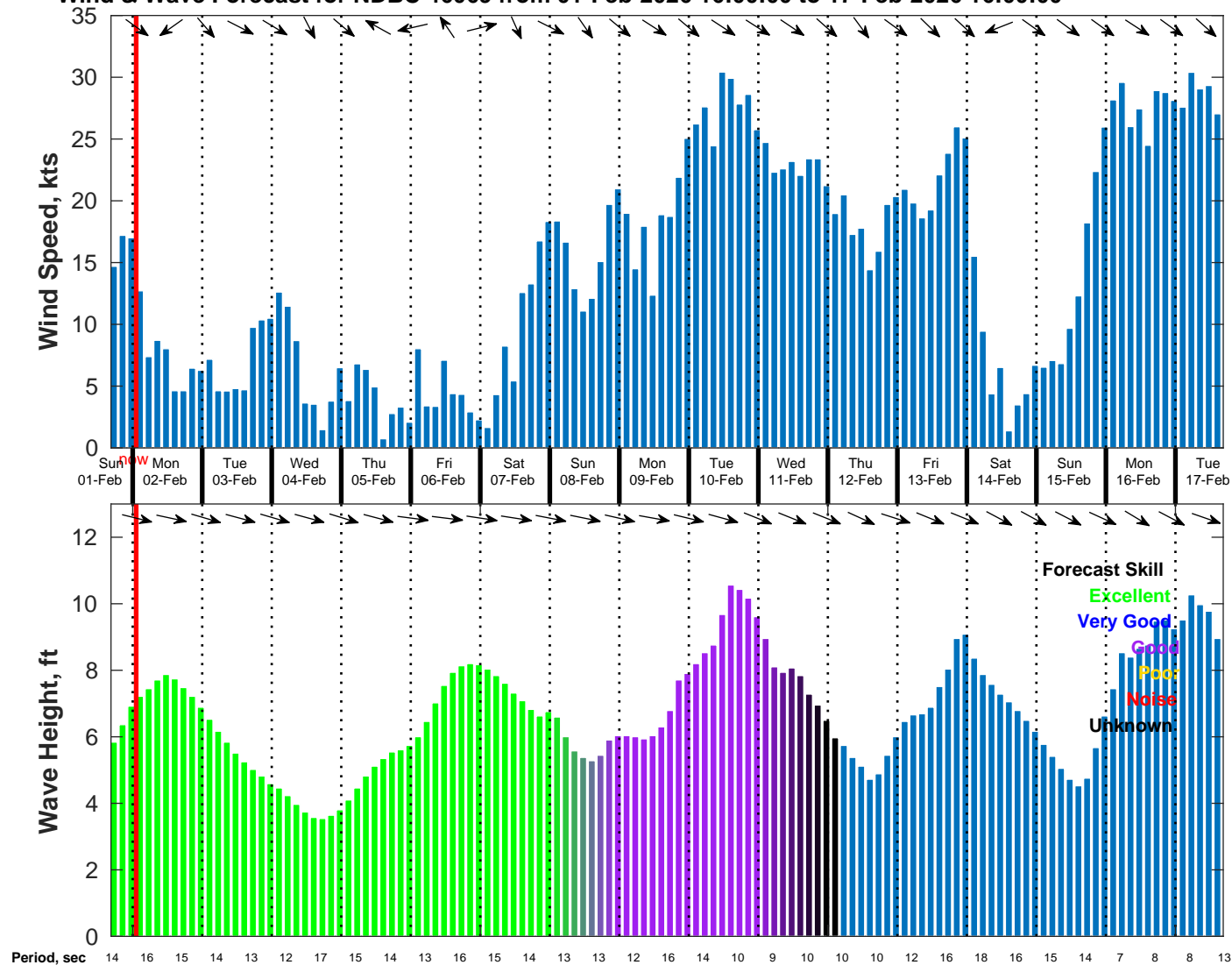
Wind & Wave Forecast for NDBC 46069 from 01-Feb-2026 16:00:00 to 17-Feb-2026 16:00:00
