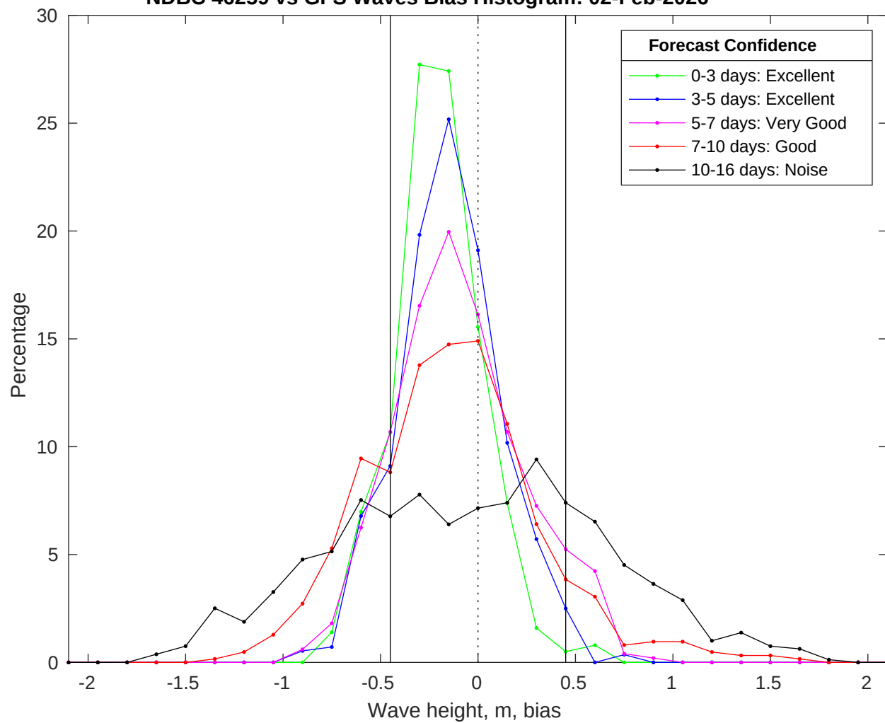
NDBC 46259 vs GFS Waves Bias Histogram: 02-Feb-2026
