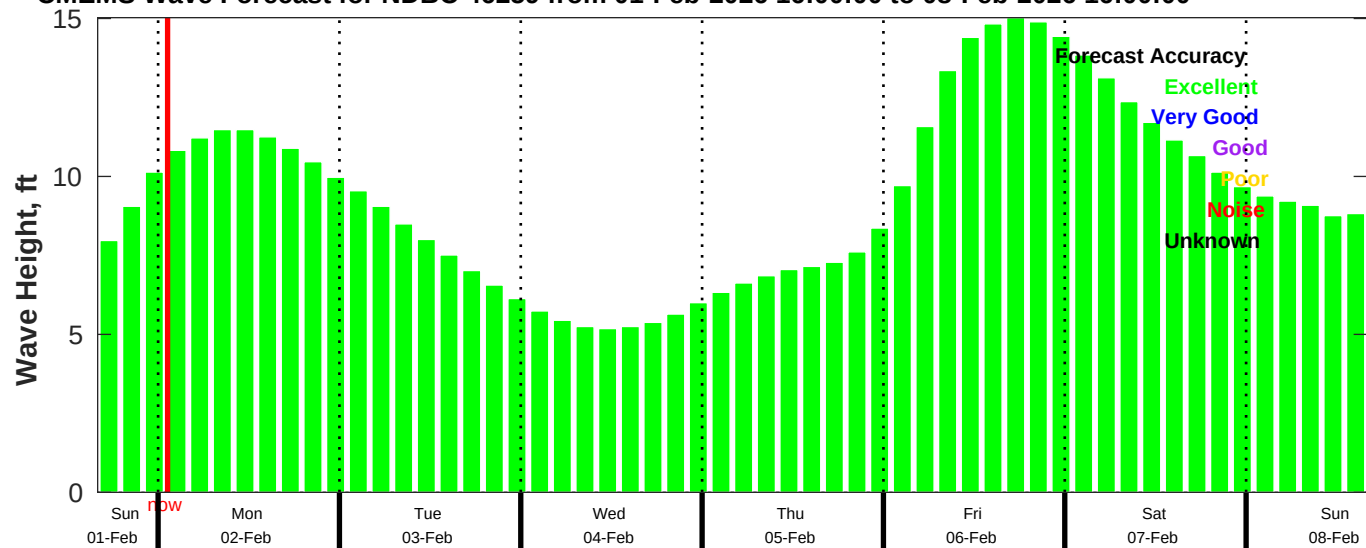
CMEMS Wave Forecast for NDBC 46259 from 01-Feb-2026 16:00:00 to 08-Feb-2026 16:00:00
