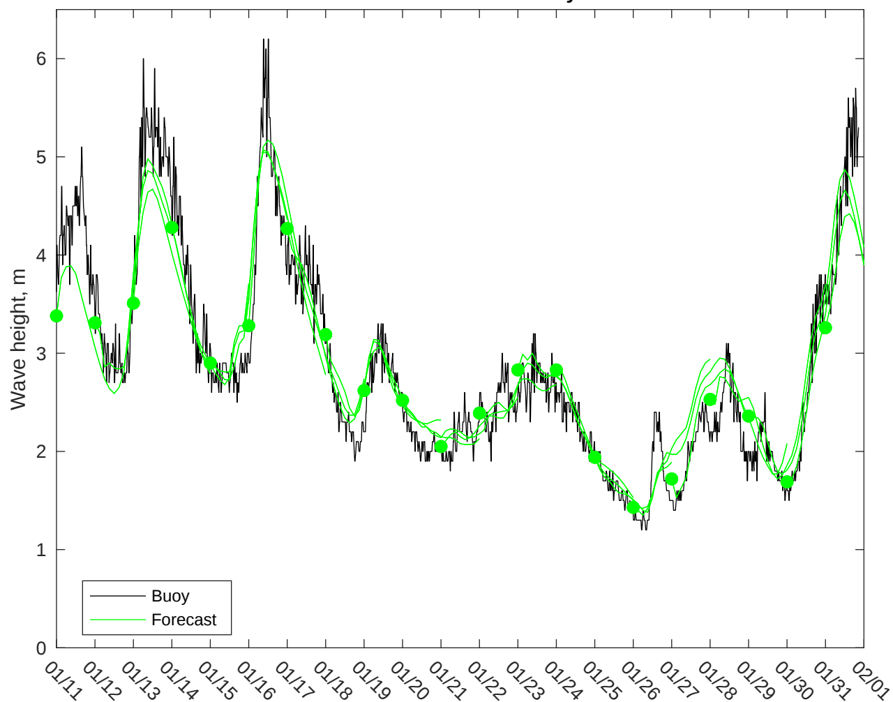
NDBC 51000 vs CMEMS Waves: 0 to 3 day forecast
