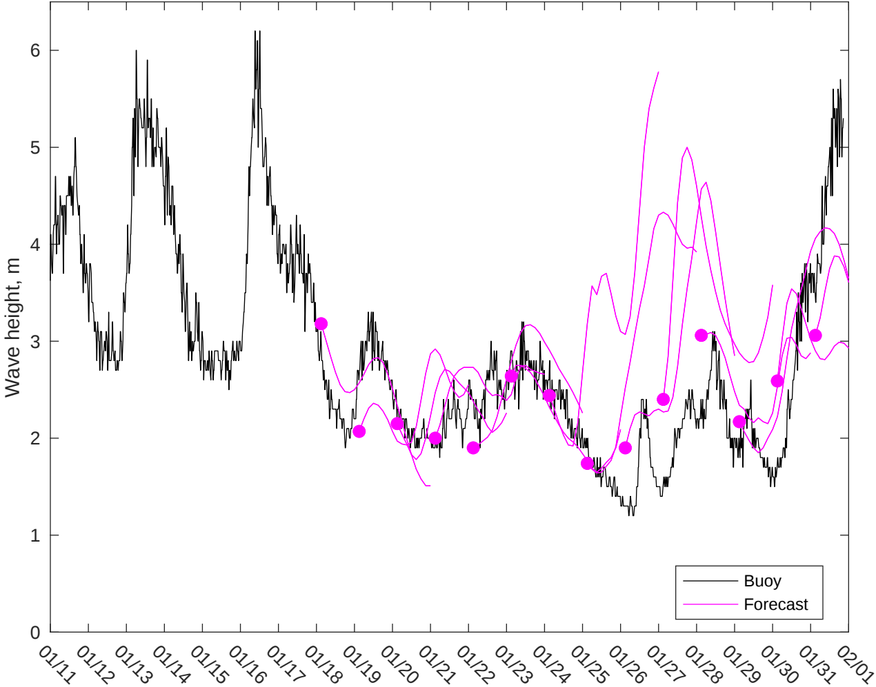
NDBC 51000 vs CMEMS Waves: 7 to 10 day forecast
