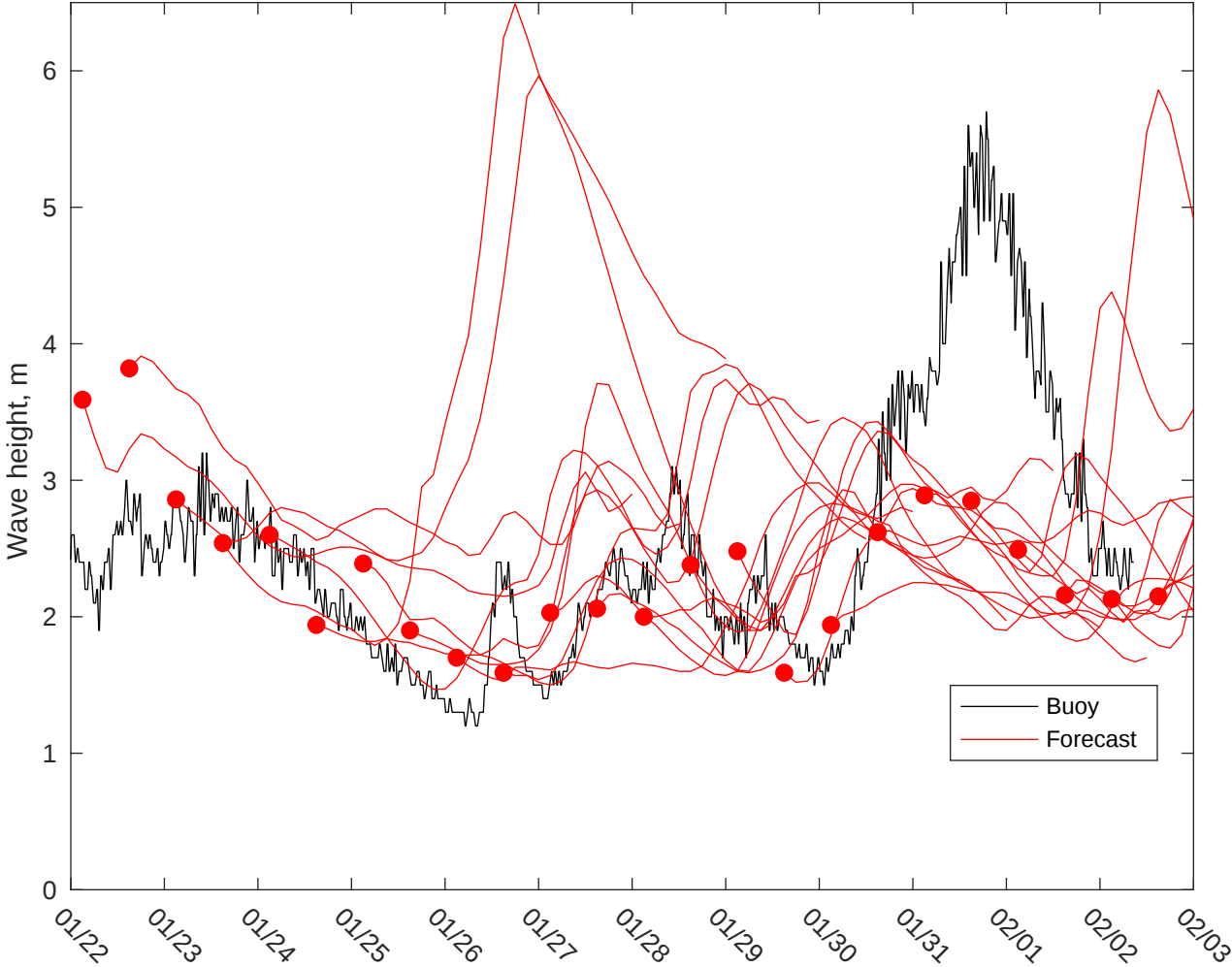
NDBC 51000 vs GFS Waves: 10 to 16 day forecast
