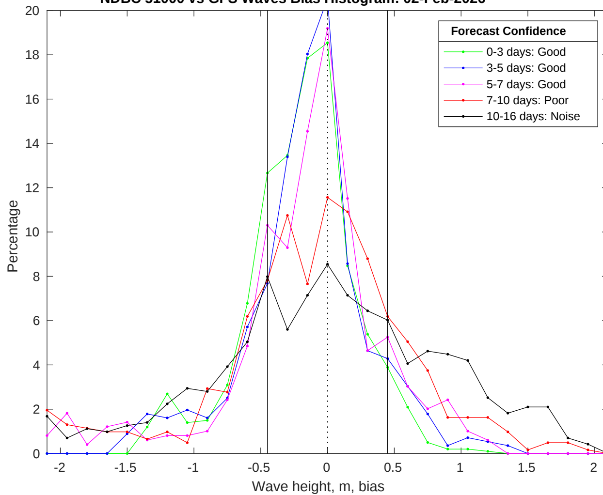
NDBC 51000 vs GFS Waves Bias Histogram: 02-Feb-2026
