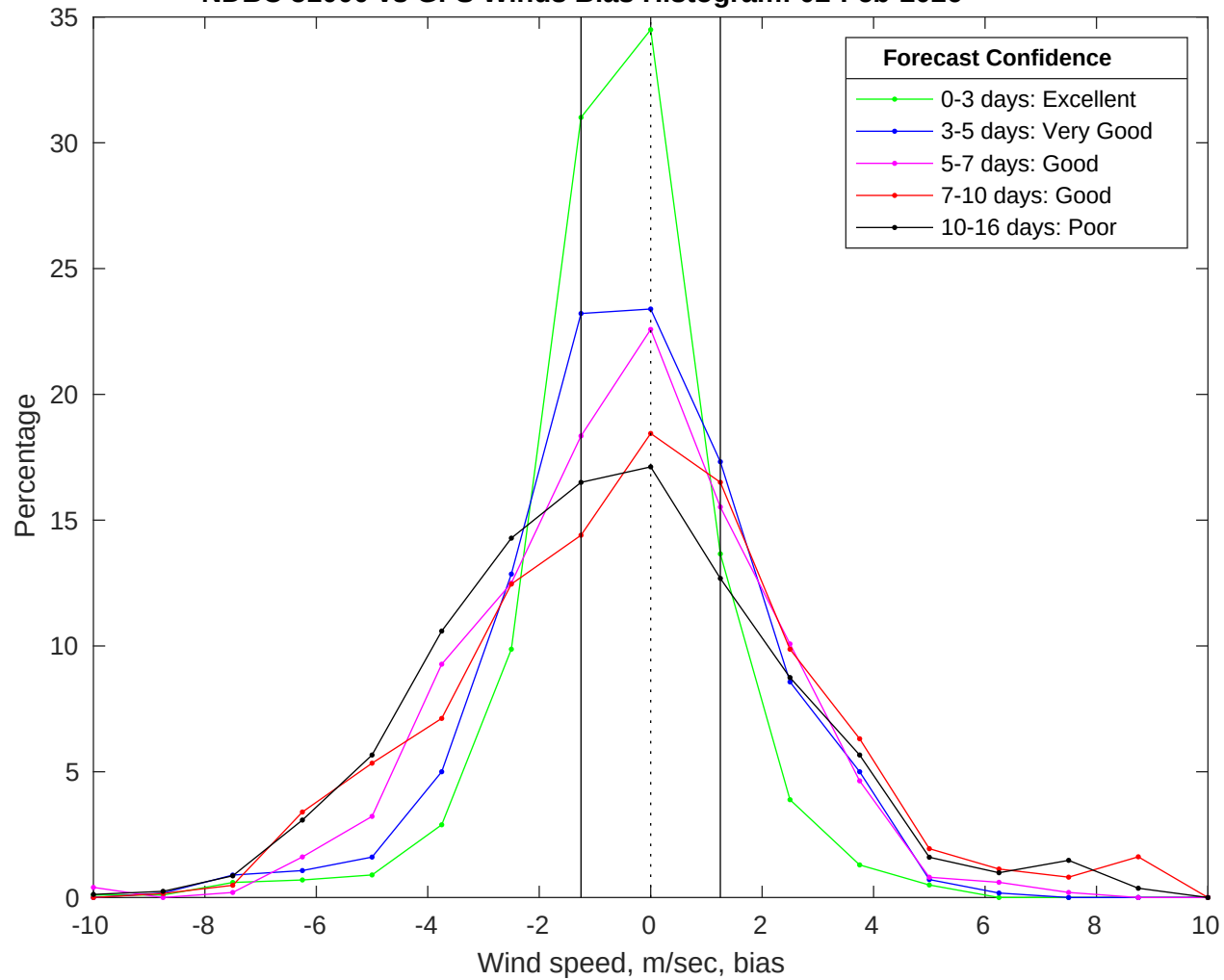
NDBC 51000 vs GFS Winds Bias Histogram: 02-Feb-2026
