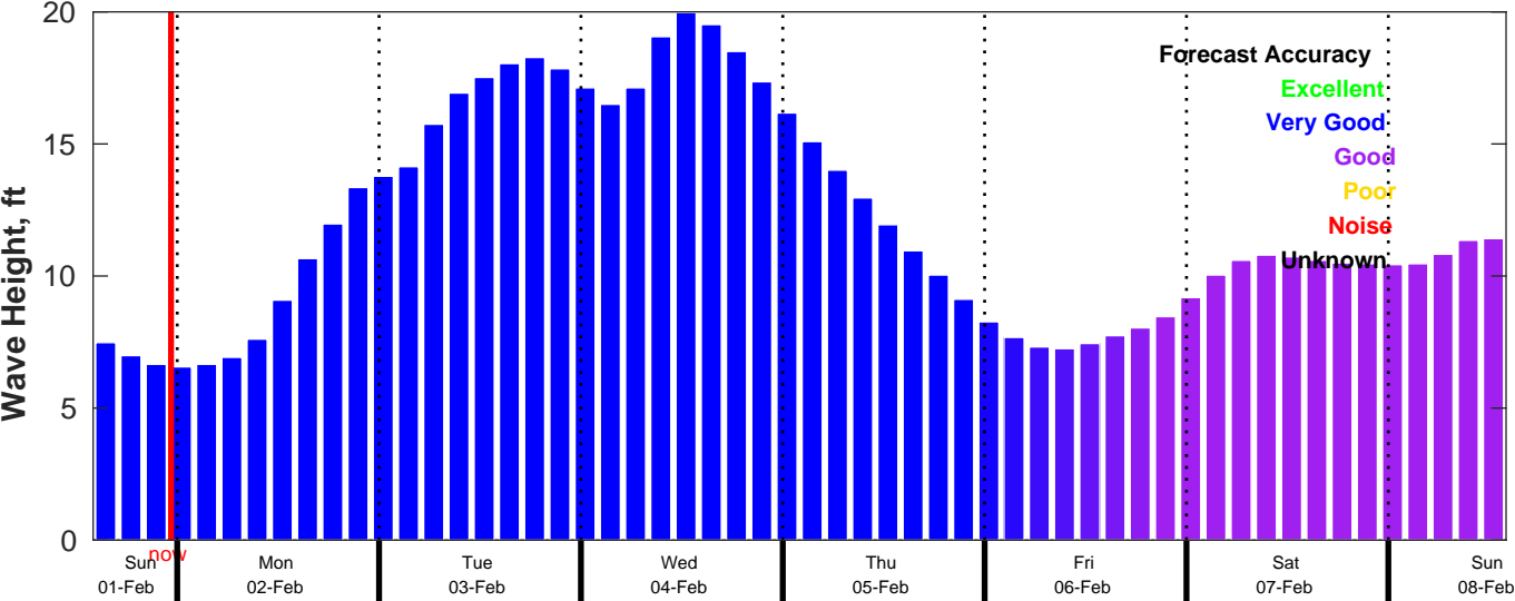
CMEMS Wave Forecast for NDBC 51000 from 01-Feb-2026 14:00:00 to 08-Feb-2026 14:00:00
