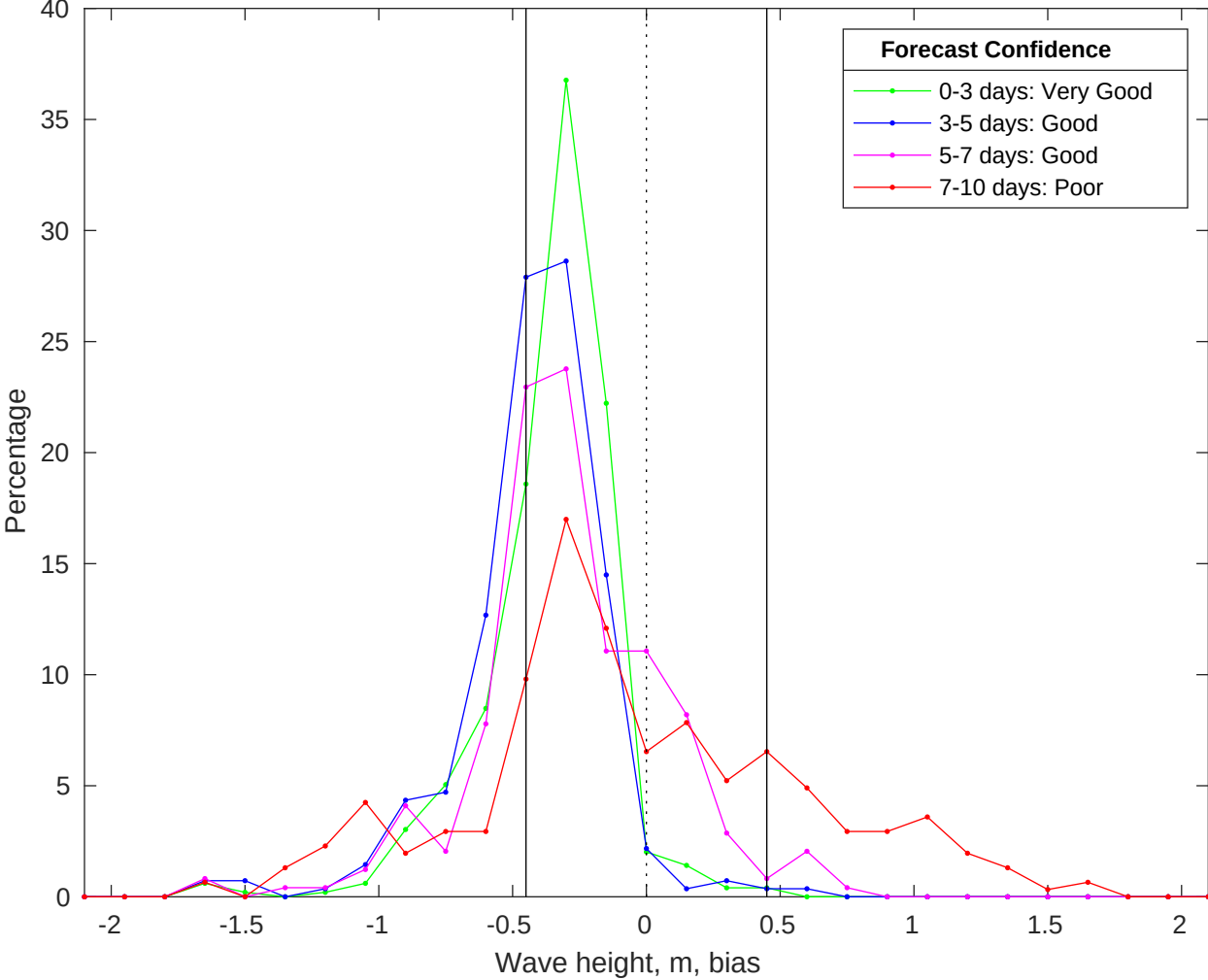
NDBC 51209 vs CMEMS Waves Bias Histogram: 31-Jan-2026
