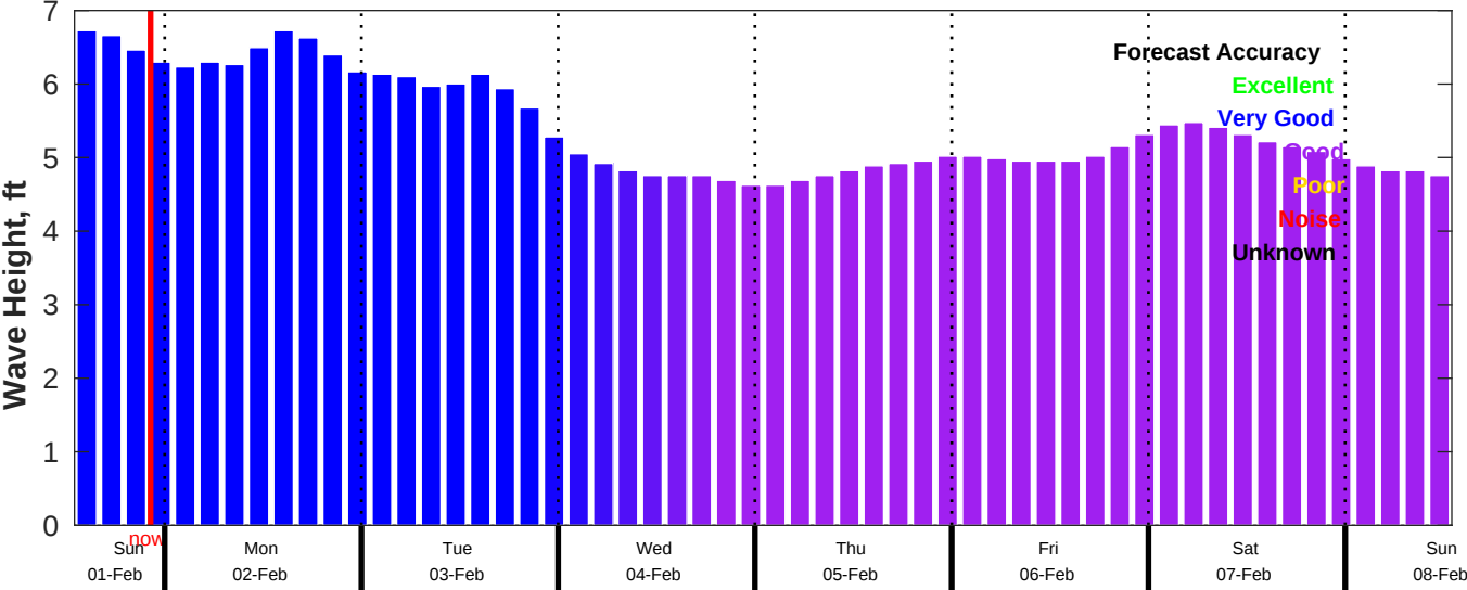
CMEMS Wave Forecast for NDBC 51209 from 01-Feb-2026 13:00:00 to 08-Feb-2026 13:00:00
