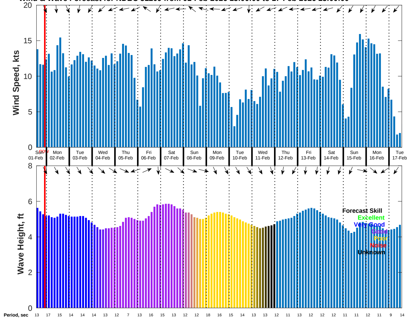
Wind & Wave Forecast for NDBC 51209 from 01-Feb-2026 13:00:00 to 17-Feb-2026 13:00:00
