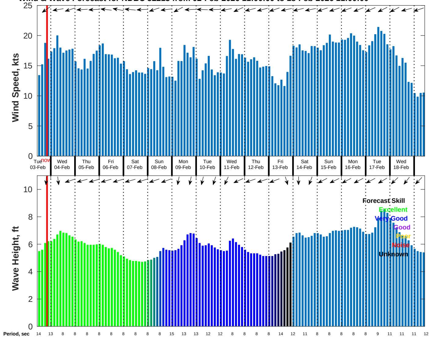
Wind & Wave Forecast for NDBC 52213 from 02-Feb-2026 11:00:00 to 18-Feb-2026 11:00:00
