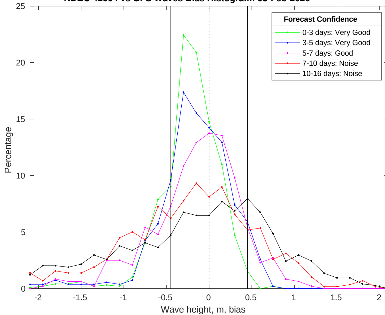
NDBC 41004 vs GFS Waves Bias Histogram: 03-Feb-2026
