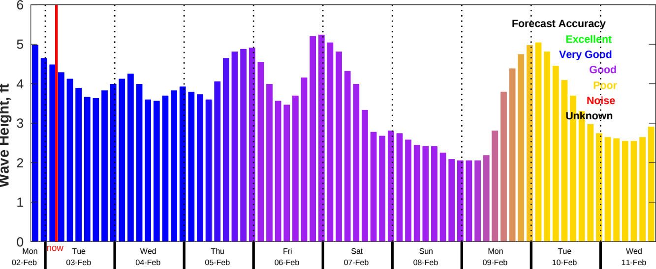
CMEMS Wave Forecast for NDBC 41004 from 02-Feb-2026 19:00:00 to 11-Feb-2026 19:00:00
