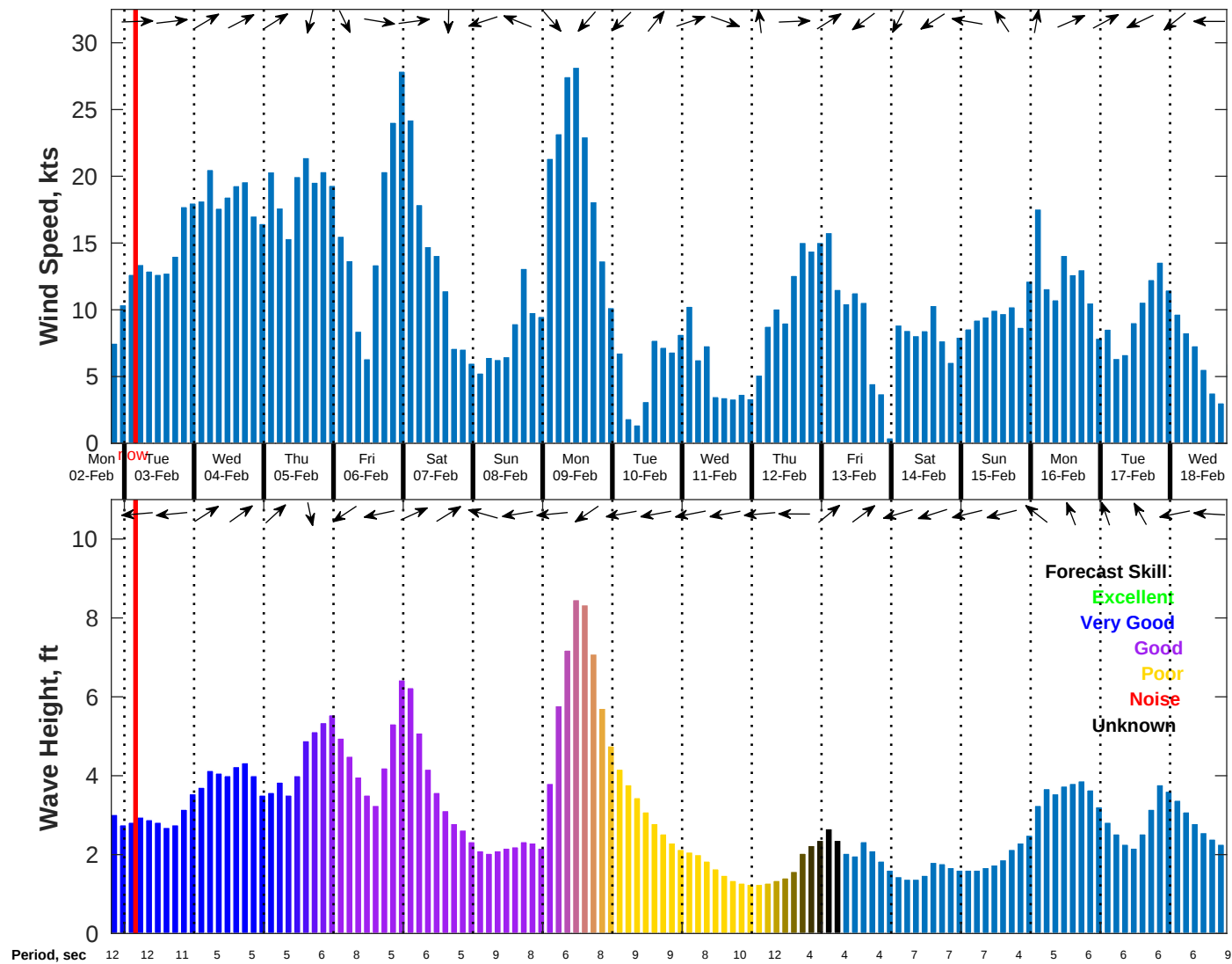
Wind & Wave Forecast for NDBC 41004 from 02-Feb-2026 19:00:00 to 18-Feb-2026 19:00:00
