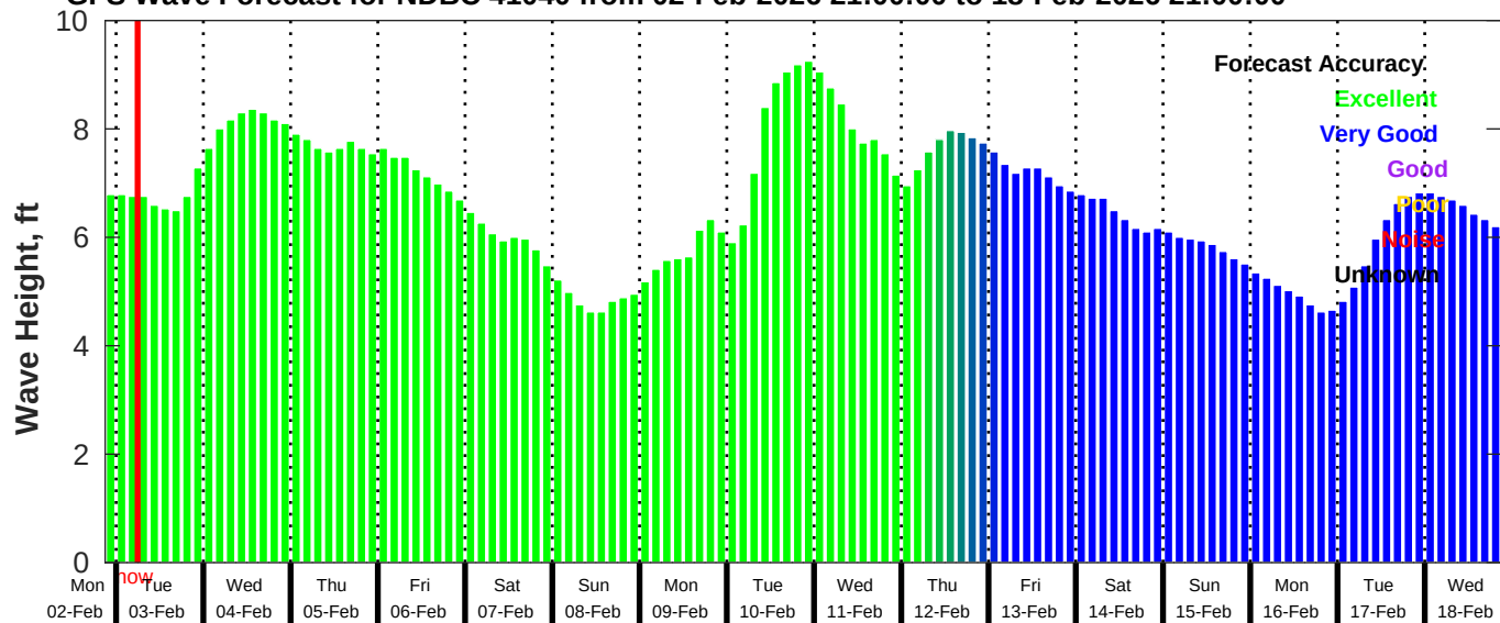
GFS Wave Forecast for NDBC 41040 from 02-Feb-2026 21:00:00 to 18-Feb-2026 21:00:00
