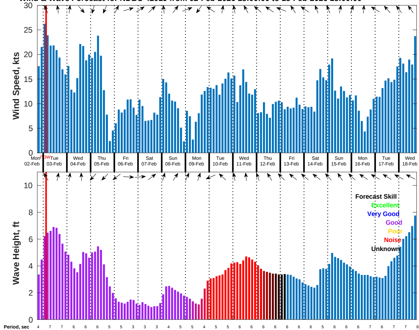
Wind & Wave Forecast for NDBC 42019 from 02-Feb-2026 18:00:00 to 18-Feb-2026 18:00:00
