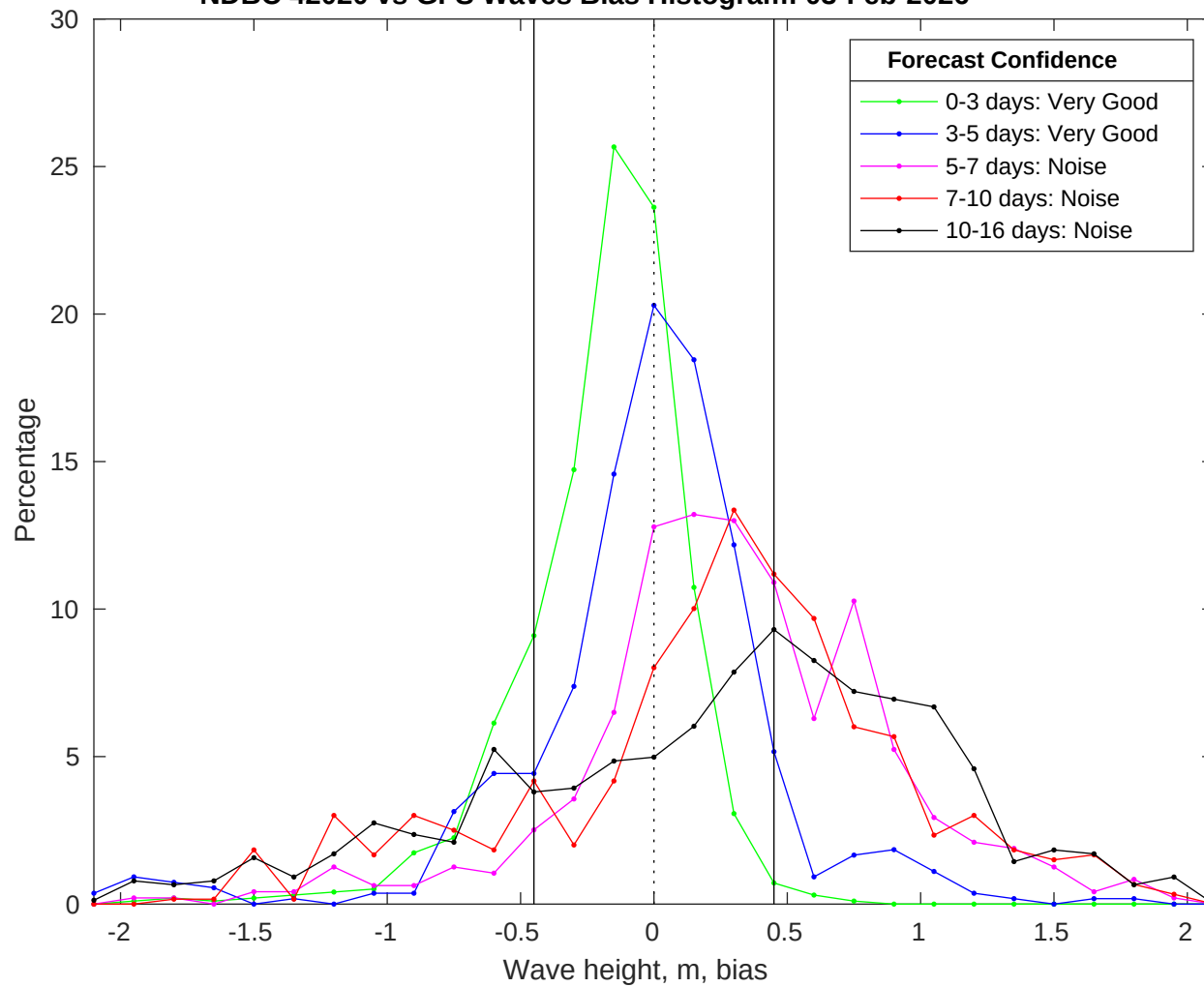
NDBC 42020 vs GFS Waves Bias Histogram: 03-Feb-2026
