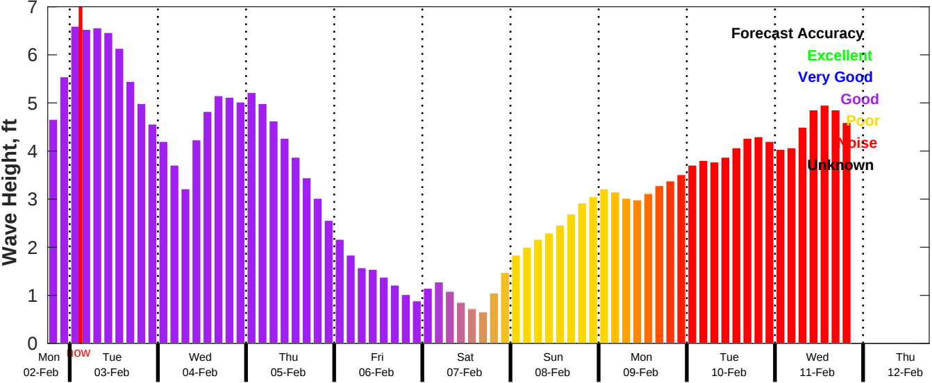
CMEMS Wave Forecast for NDBC 42020 from 02-Feb-2026 18:00:00 to 12-Feb-2026 18:00:00
