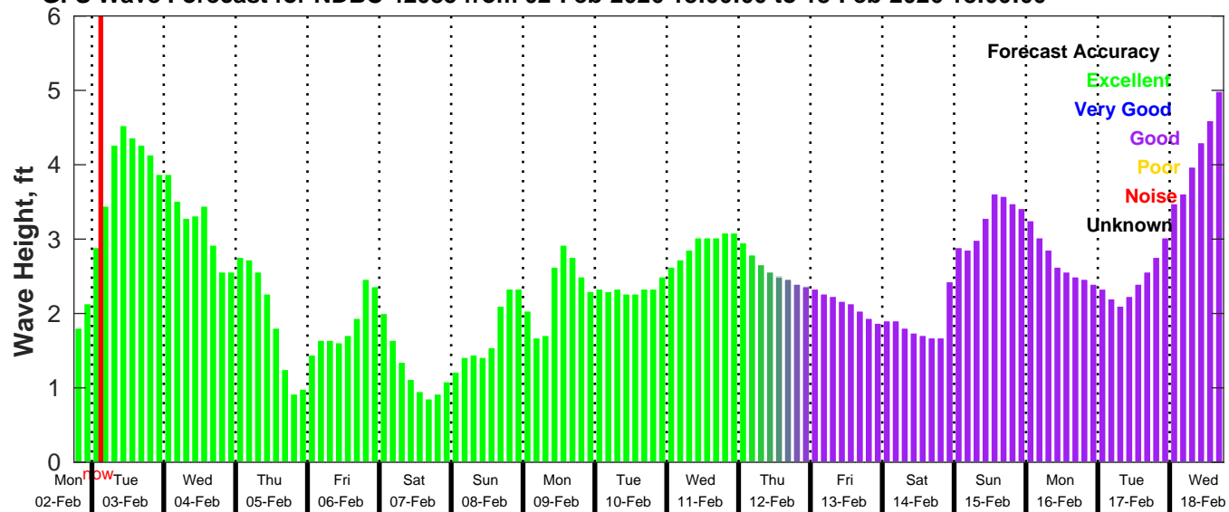
GFS Wave Forecast for NDBC 42035 from 02-Feb-2026 18:00:00 to 18-Feb-2026 18:00:00
