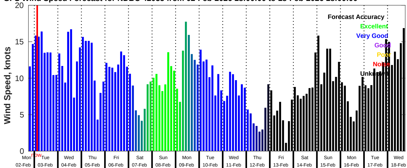
GFS Wind Speed Forecast for NDBC 42035 from 02-Feb-2026 18:00:00 to 18-Feb-2026 18:00:00
