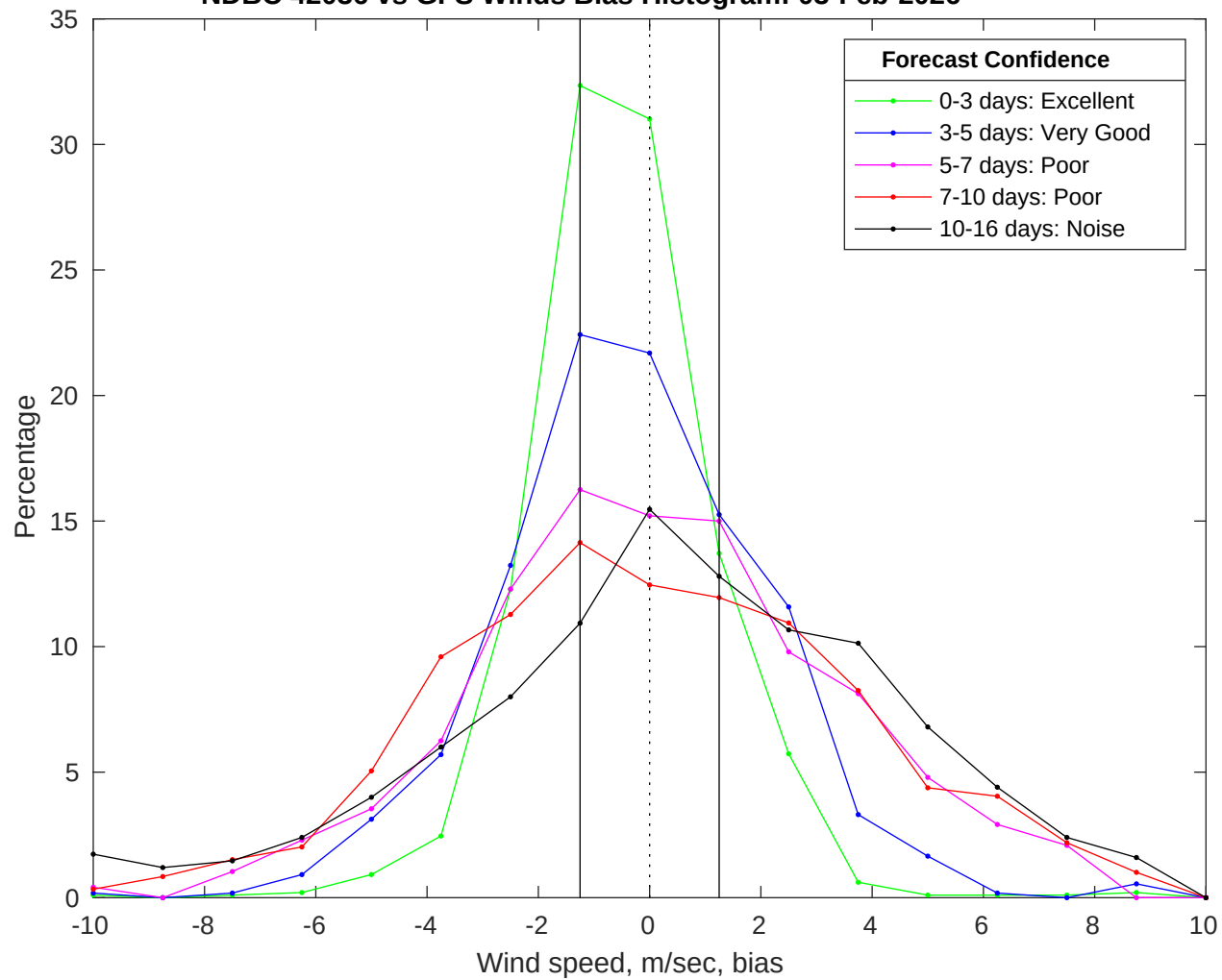
NDBC 42036 vs GFS Winds Bias Histogram: 03-Feb-2026
