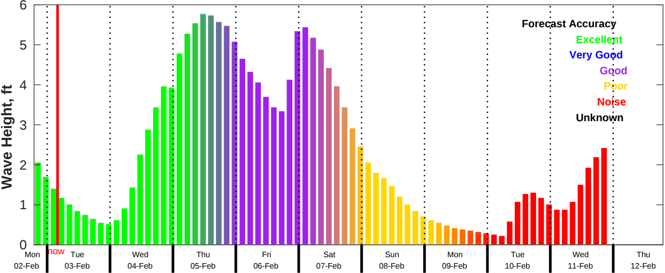
CMEMS Wave Forecast for NDBC 42036 from 02-Feb-2026 19:00:00 to 12-Feb-2026 19:00:00
