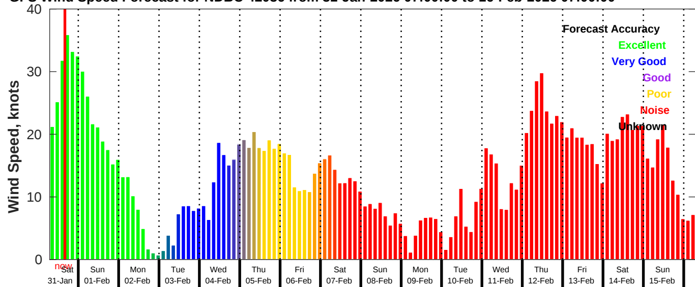
GFS Wind Speed Forecast for NDBC 42036 from 31-Jan-2026 07:00:00 to 16-Feb-2026 07:00:00
