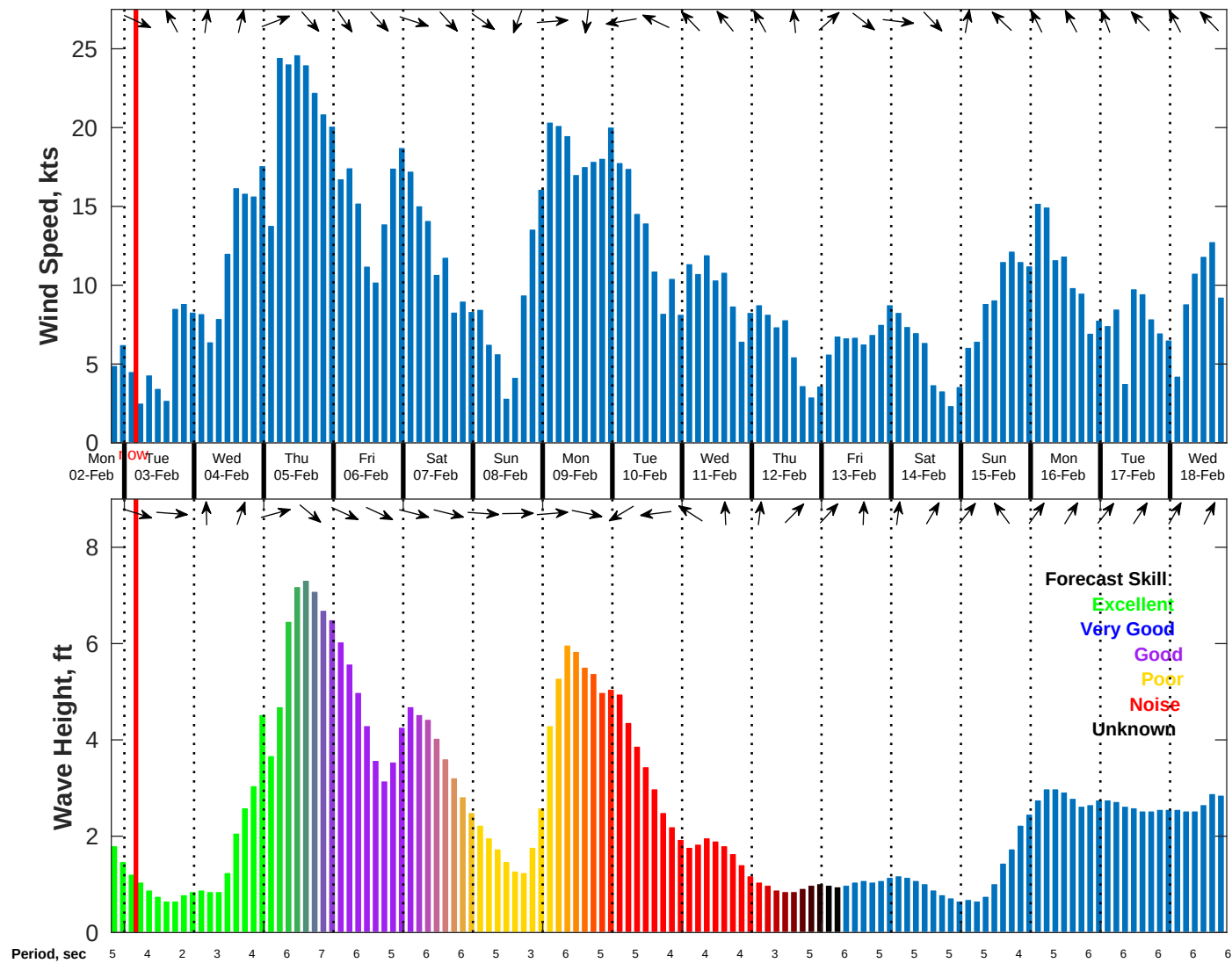
Wind & Wave Forecast for NDBC 42036 from 02-Feb-2026 19:00:00 to 18-Feb-2026 19:00:00
