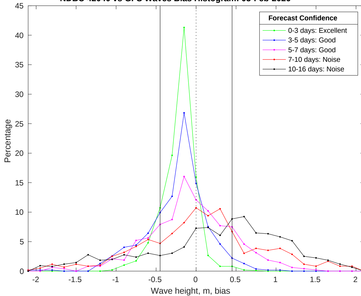
NDBC 42040 vs GFS Waves Bias Histogram: 03-Feb-2026
