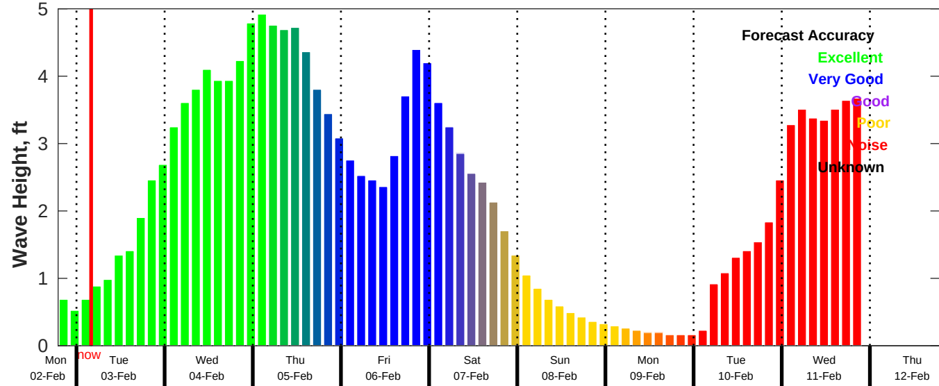
CMEMS Wave Forecast for NDBC 42040 from 02-Feb-2026 19:00:00 to 12-Feb-2026 19:00:00
