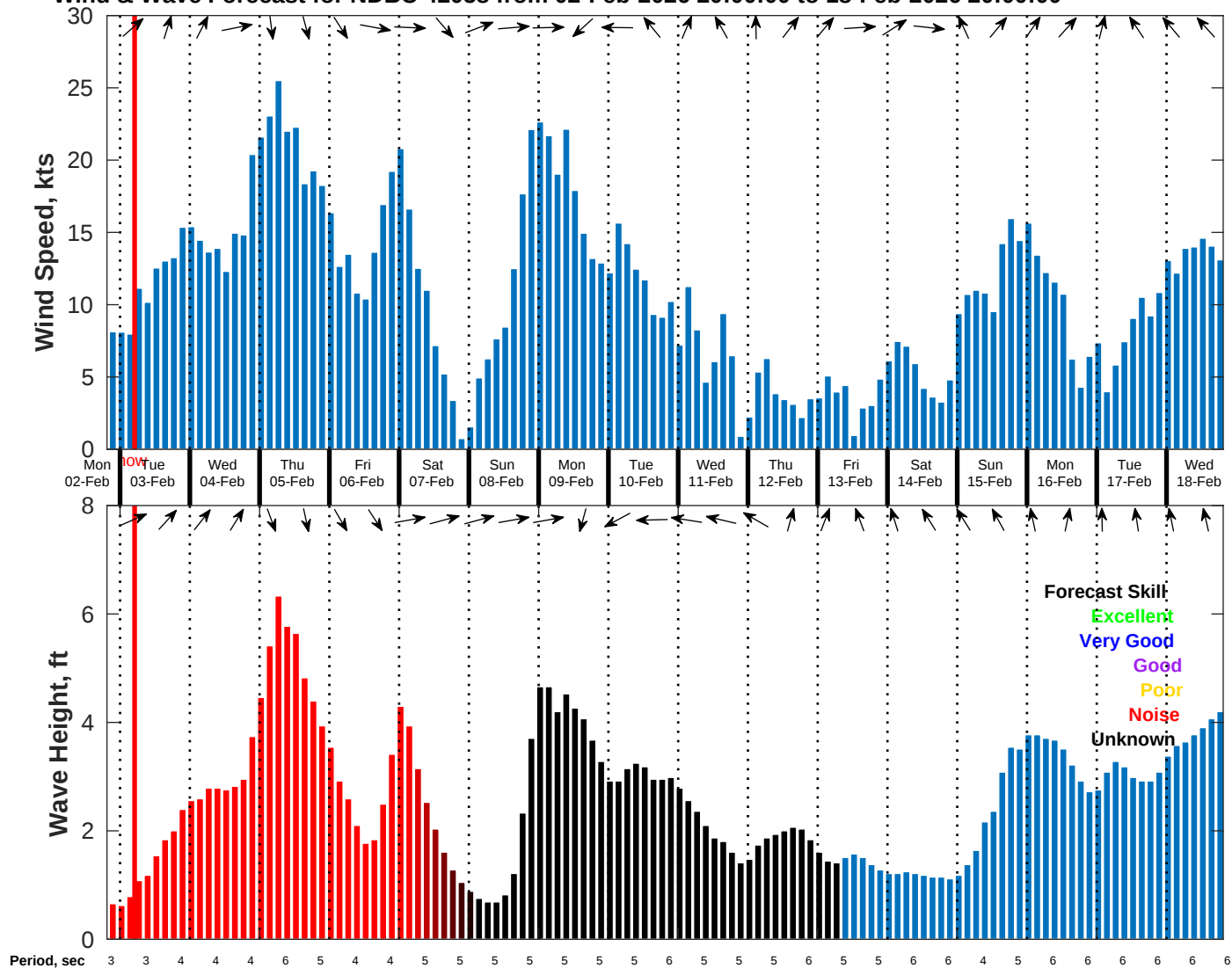
Wind & Wave Forecast for NDBC 42058 from 02-Feb-2026 20:00:00 to 18-Feb-2026 20:00:00
