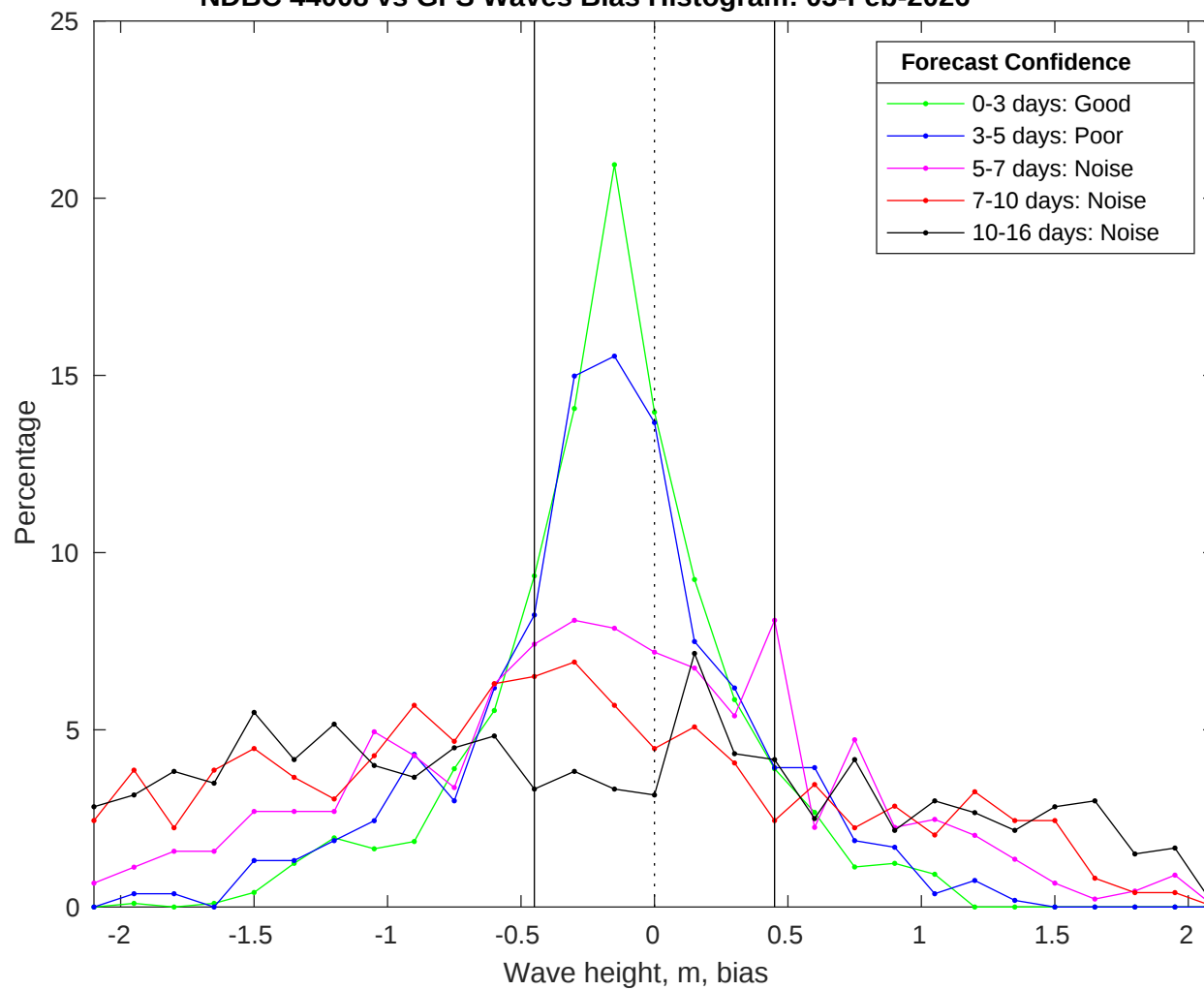
NDBC 44008 vs GFS Waves Bias Histogram: 03-Feb-2026
