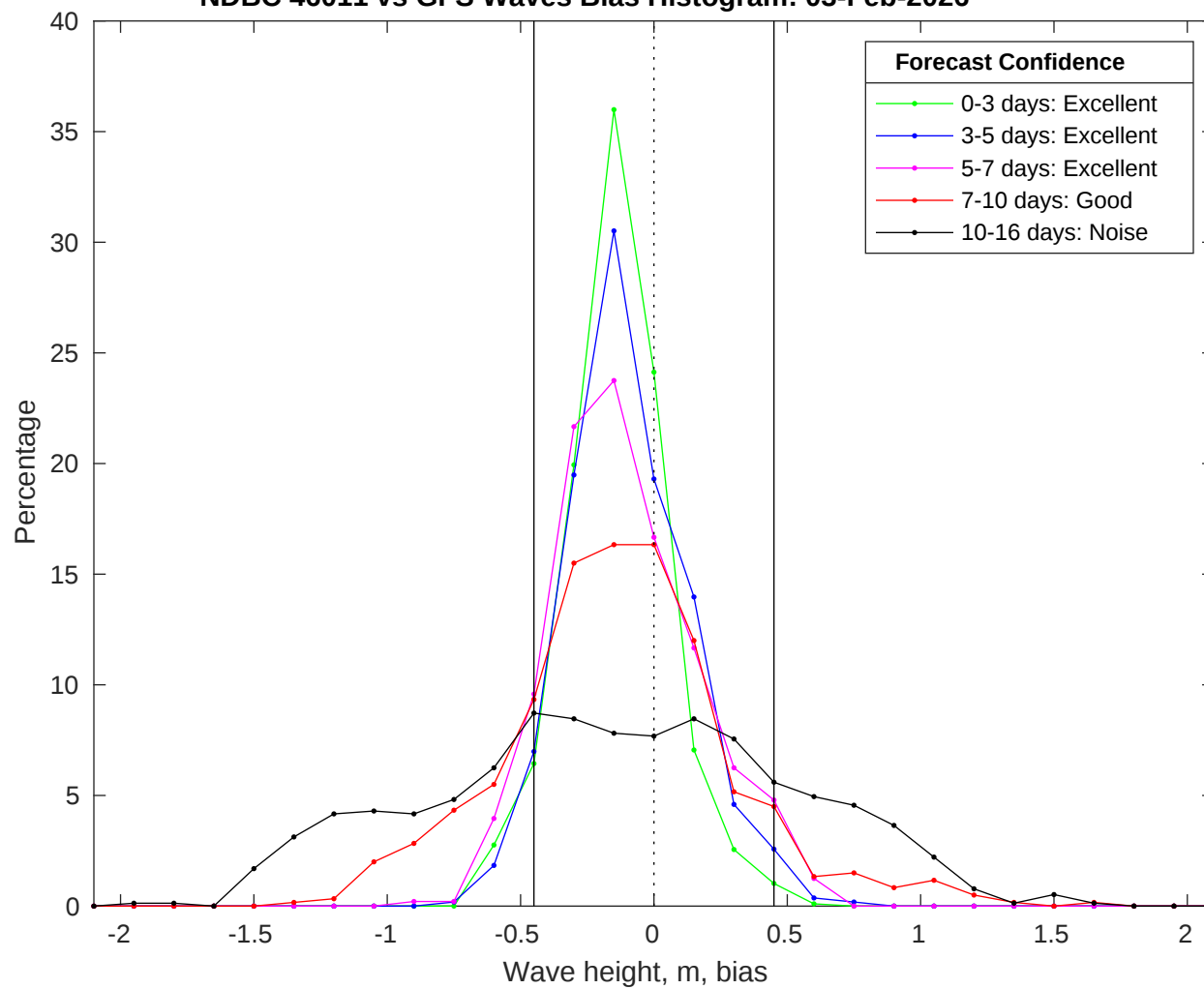
NDBC 46011 vs GFS Waves Bias Histogram: 03-Feb-2026
