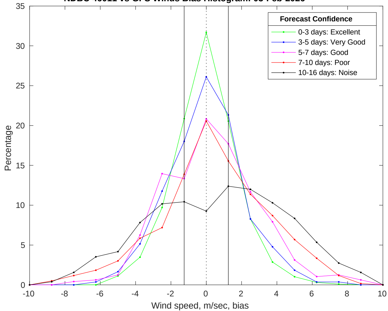
NDBC 46011 vs GFS Winds Bias Histogram: 03-Feb-2026
