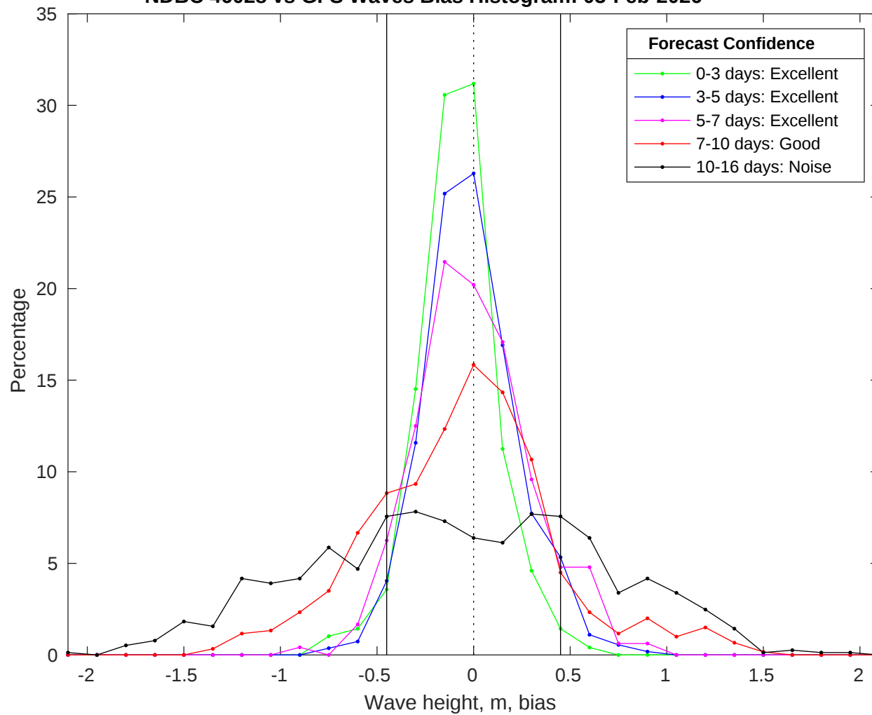
NDBC 46028 vs GFS Waves Bias Histogram: 03-Feb-2026
