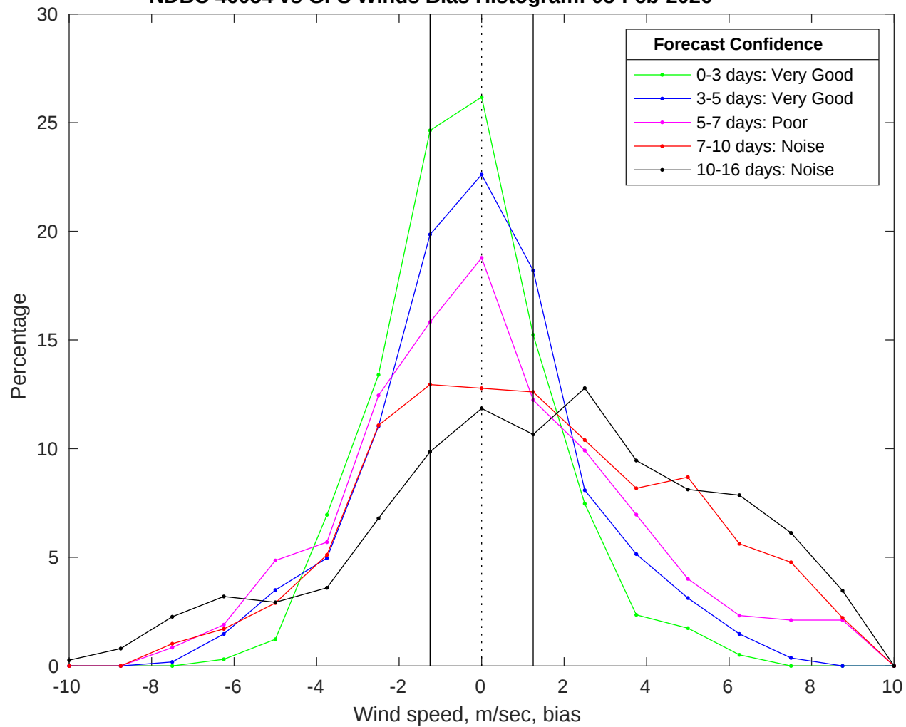
NDBC 46054 vs GFS Winds Bias Histogram: 03-Feb-2026
