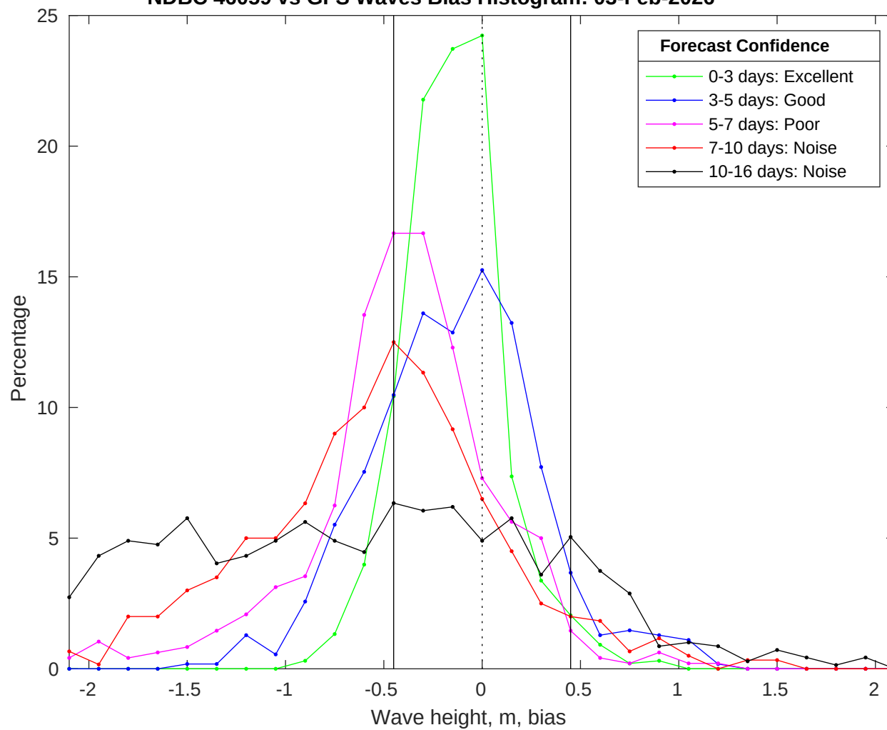
NDBC 46059 vs GFS Waves Bias Histogram: 03-Feb-2026
