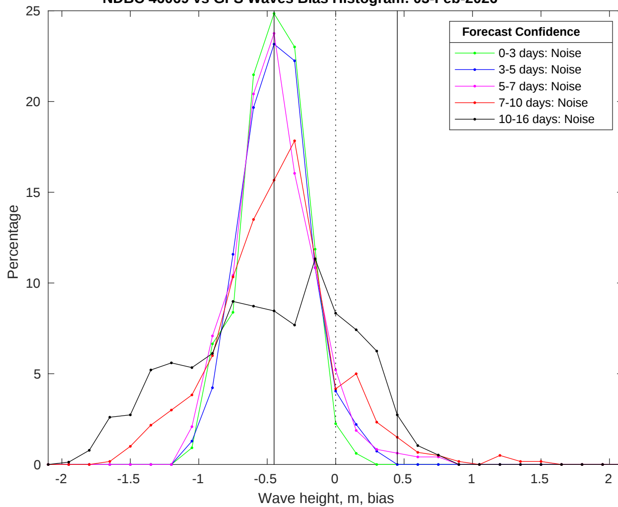
NDBC 46069 vs GFS Waves Bias Histogram: 03-Feb-2026
