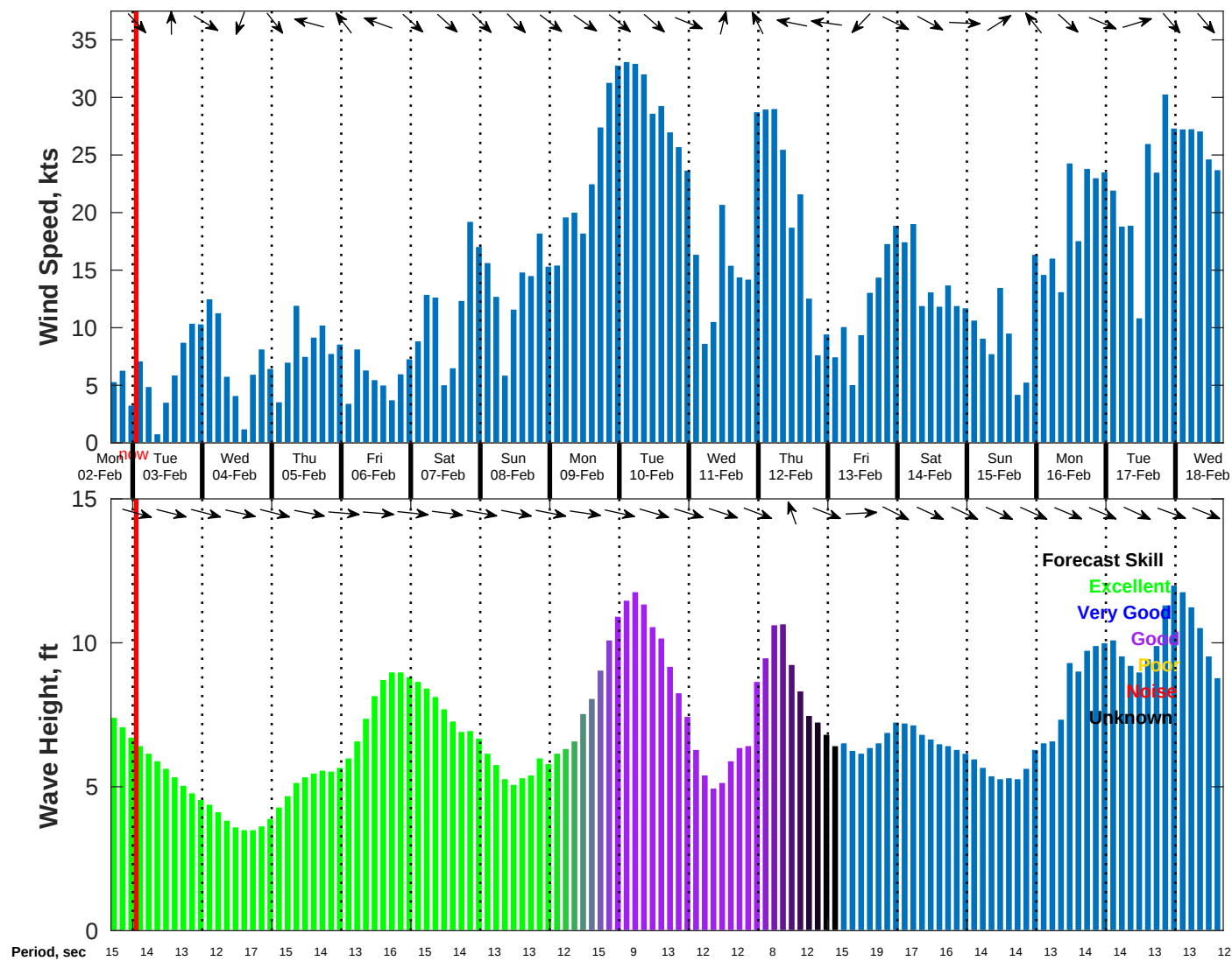
Wind & Wave Forecast for NDBC 46069 from 02-Feb-2026 16:00:00 to 18-Feb-2026 16:00:00
