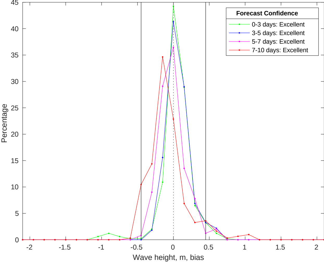
NDBC 46215 vs CMEMS Waves Bias Histogram: 31-Jan-2026
