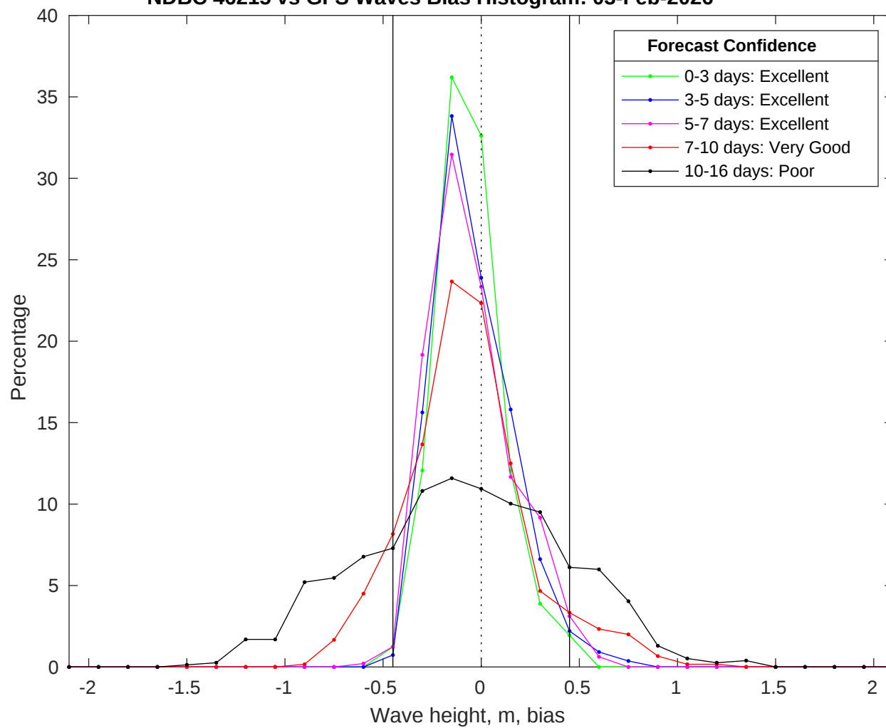
NDBC 46215 vs GFS Waves Bias Histogram: 03-Feb-2026
