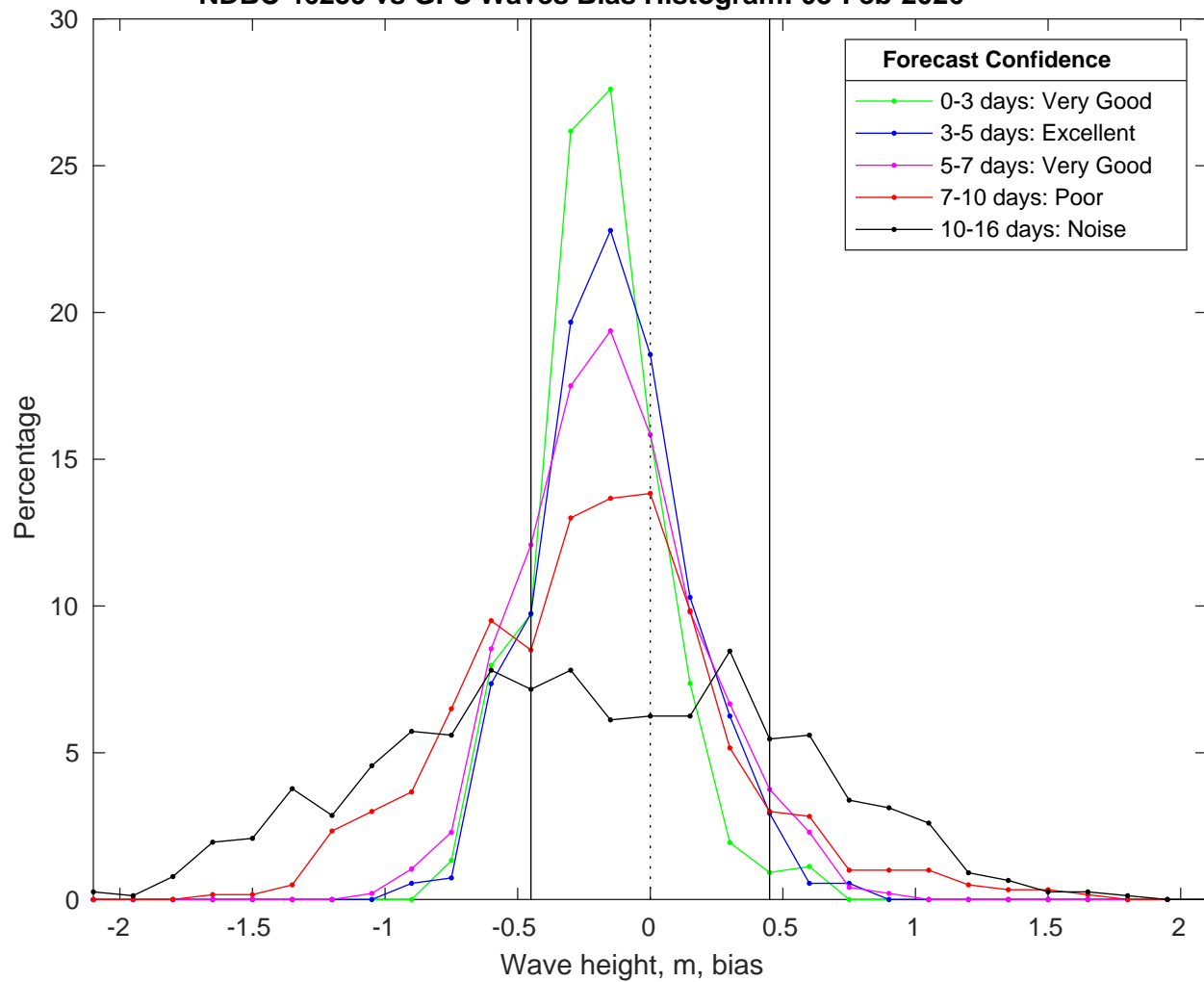
NDBC 46259 vs GFS Waves Bias Histogram: 03-Feb-2026
