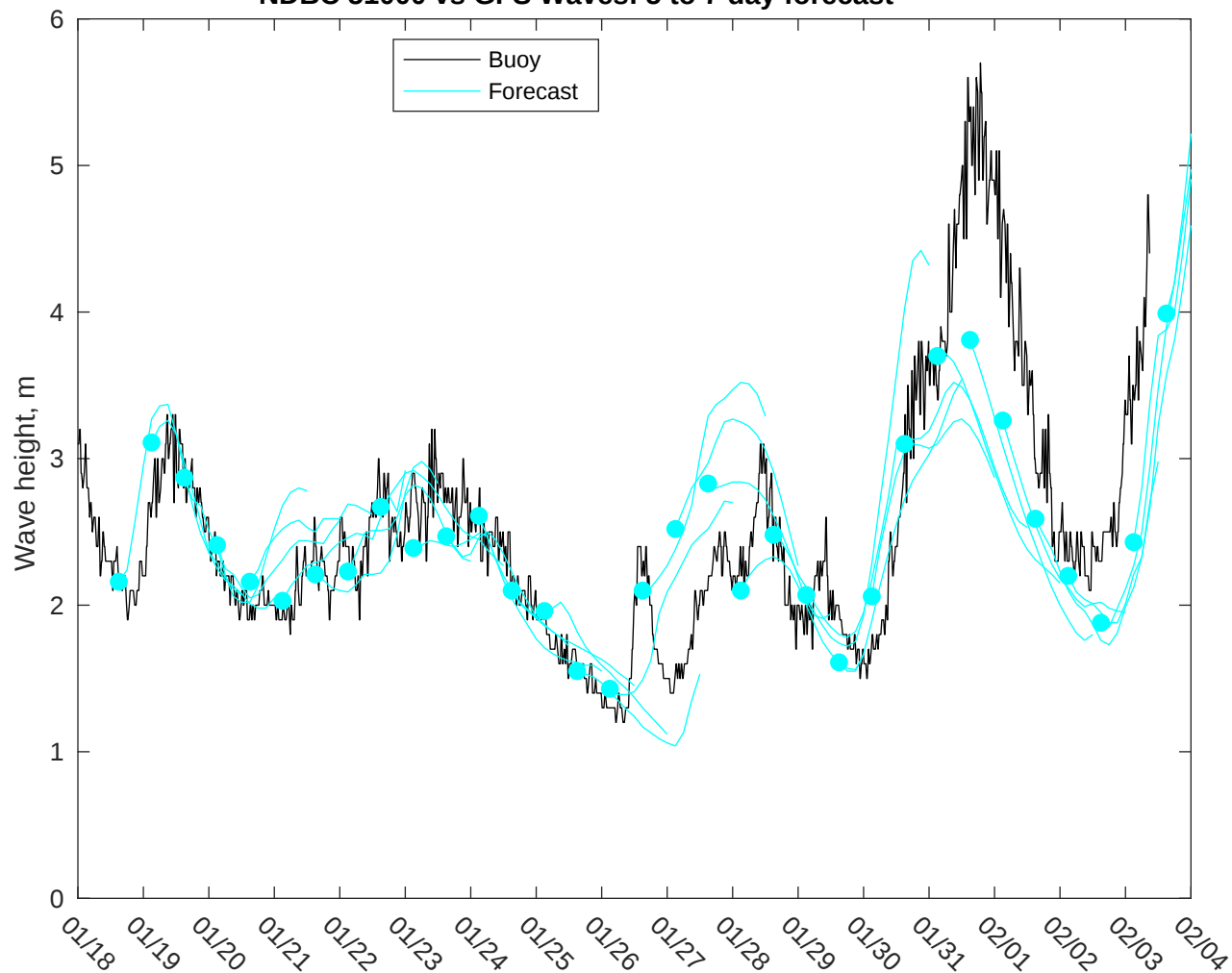
NDBC 51000 vs GFS Waves: 5 to 7 day forecast
