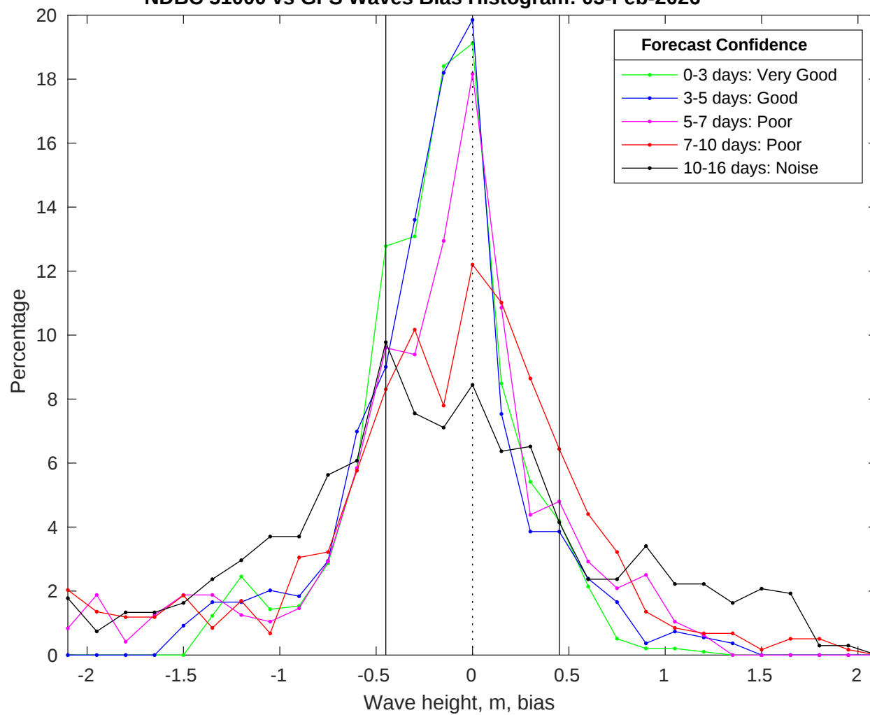
NDBC 51000 vs GFS Waves Bias Histogram: 03-Feb-2026
