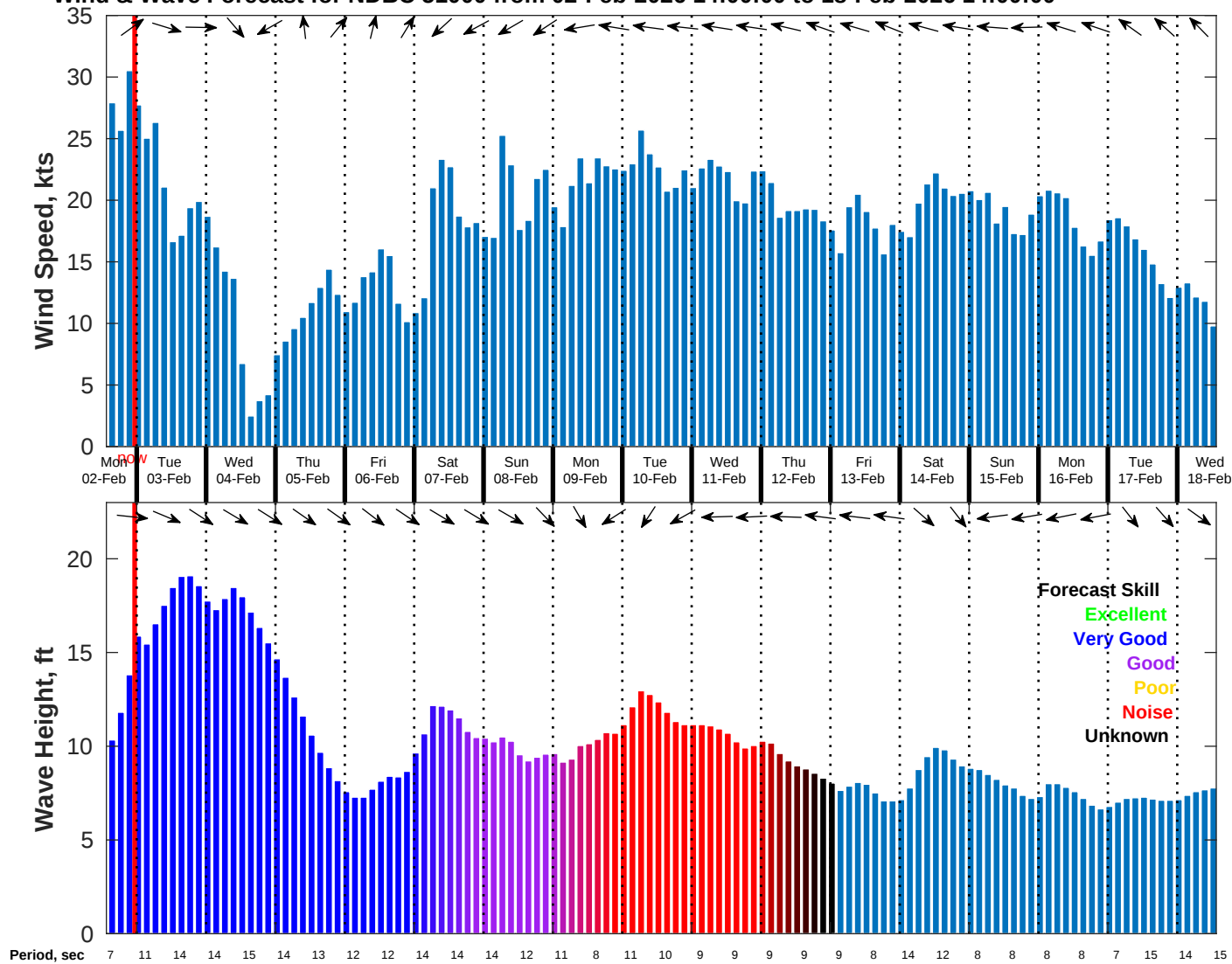
Wind & Wave Forecast for NDBC 51000 from 02-Feb-2026 14:00:00 to 18-Feb-2026 14:00:00
