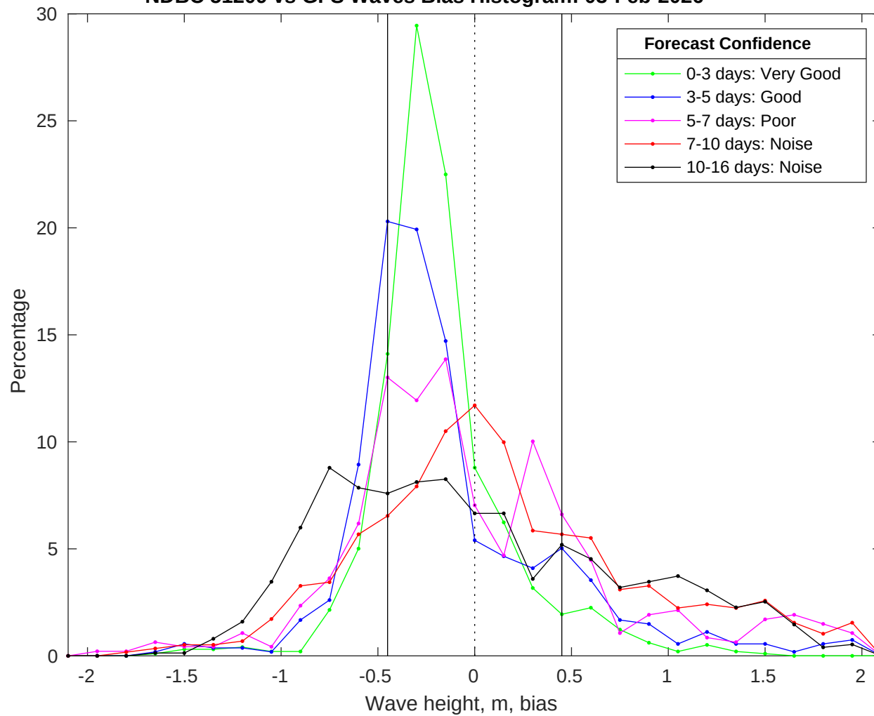
NDBC 51209 vs GFS Waves Bias Histogram: 03-Feb-2026
